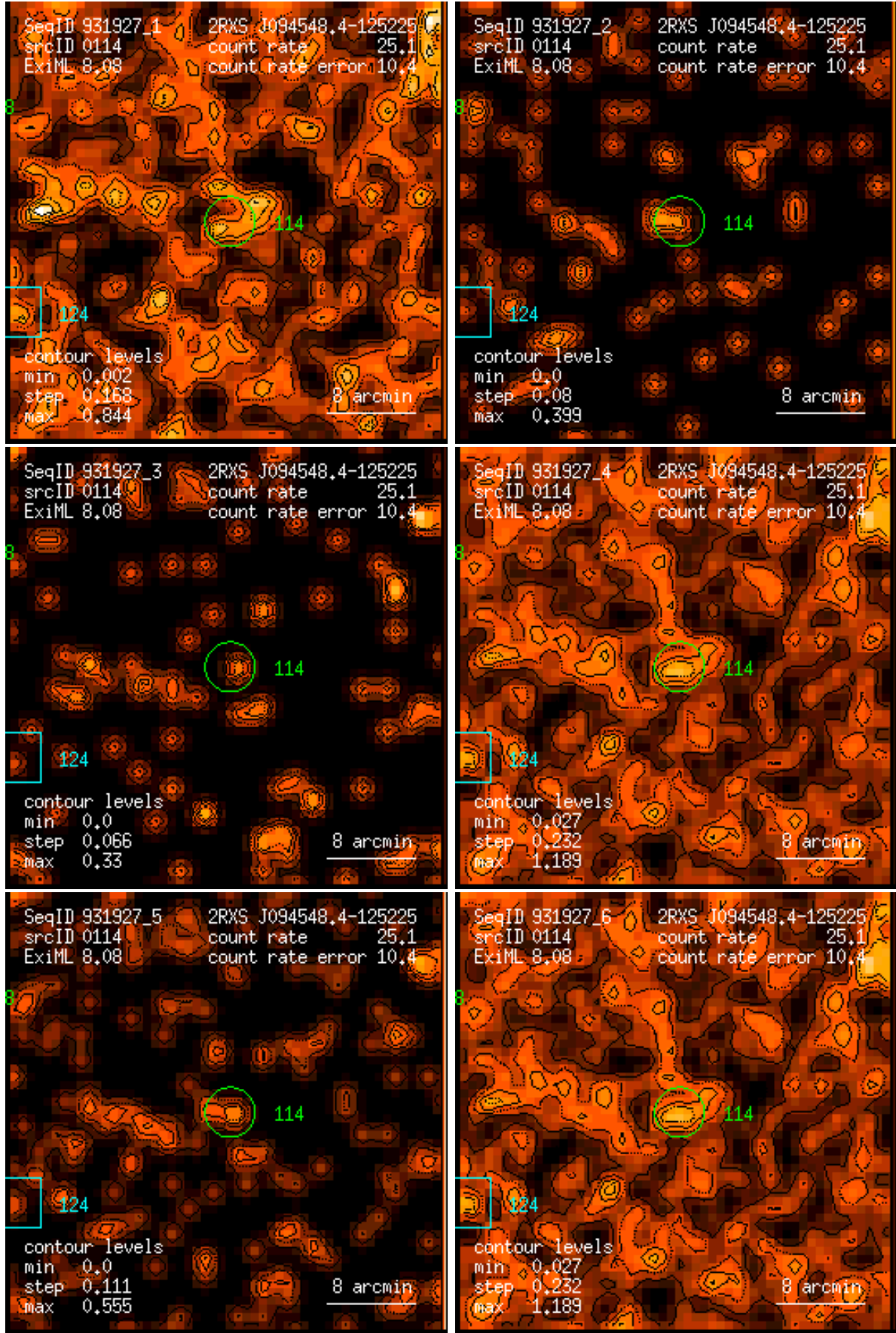
Figure 114: RASS 931927: detection 0114: band rate images, Gaussian filter: (1) PSPC channels 11 – 41, (2) 52 – 90, (3) 91 – 201, (4) 11 – 235, (5) 52 – 201, (6) 11 – 201. Broad band rates in counts/ks. Band rate contour levels in counts/ks/arcmin 2 .
