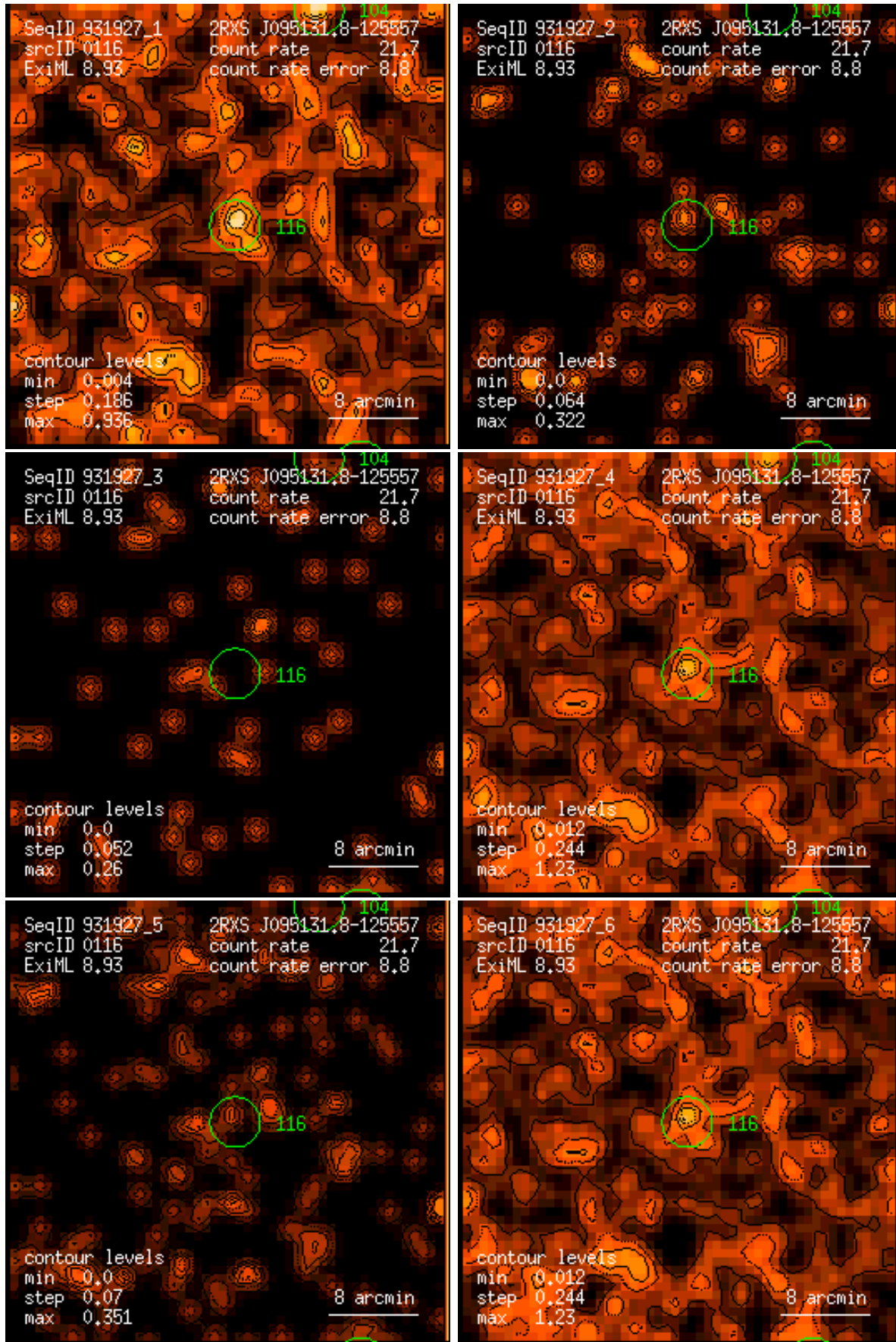
Figure 116: RASS 931927: detection 0116: band rate images, Gaussian filter: (1) PSPC channels 11 – 41, (2) 52 – 90, (3) 91 – 201, (4) 11 – 235, (5) 52 – 201, (6) 11 – 201. Broad band rates in counts/ks. Band rate contour levels in counts/ks/arcmin 2 .
