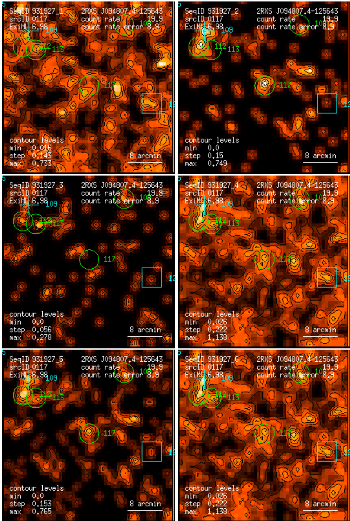
Figure 117: RASS 931927: detection 0117: band rate images, Gaussian filter: (1) PSPC channels 11 – 41, (2) 52 – 90, (3) 91 – 201, (4) 11 – 235, (5) 52 – 201, (6) 11 – 201. Broad band rates in counts/ks. Band rate contour levels in counts/ks/arcmin 2 .
