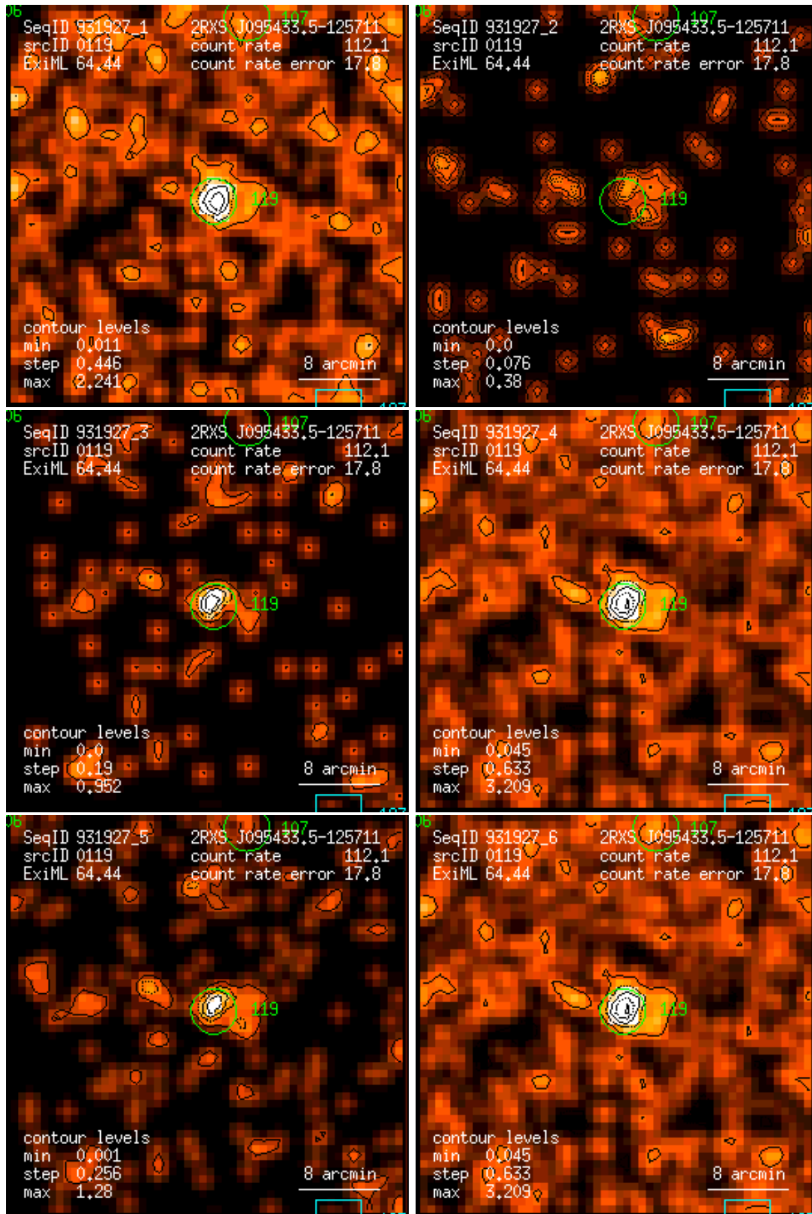
Figure 119: RASS 931927: detection 0119: band rate images, Gaussian filter: (1) PSPC channels 11 – 41, (2) 52 – 90, (3) 91 – 201, (4) 11 – 235, (5) 52 – 201, (6) 11 – 201. Broad band rates in counts/ks. Band rate contour levels in counts/ks/arcmin 2 .
