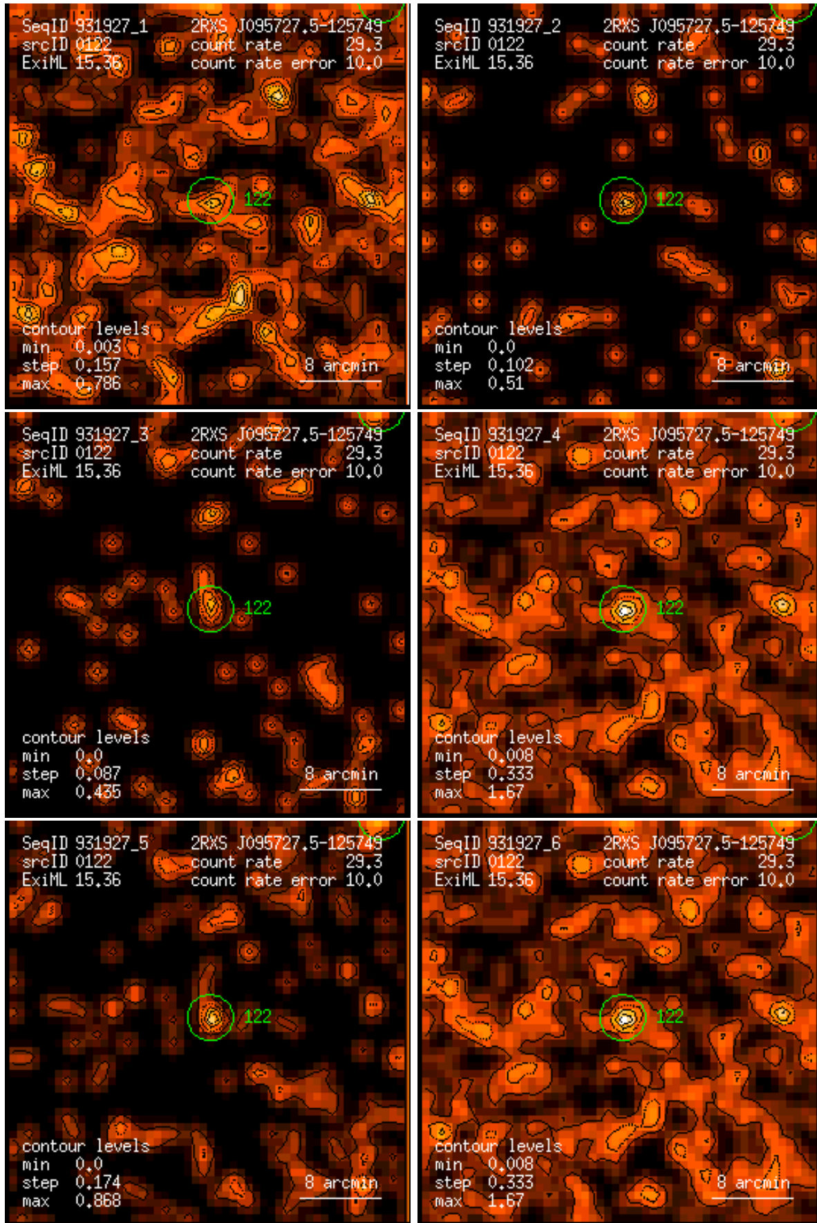
Figure 122: RASS 931927: detection 0122: band rate images, Gaussian filter: (1) PSPC channels 11 – 41, (2) 52 – 90, (3) 91 – 201, (4) 11 – 235, (5) 52 – 201, (6) 11 – 201. Broad band rates in counts/ks. Band rate contour levels in counts/ks/arcmin 2 .
