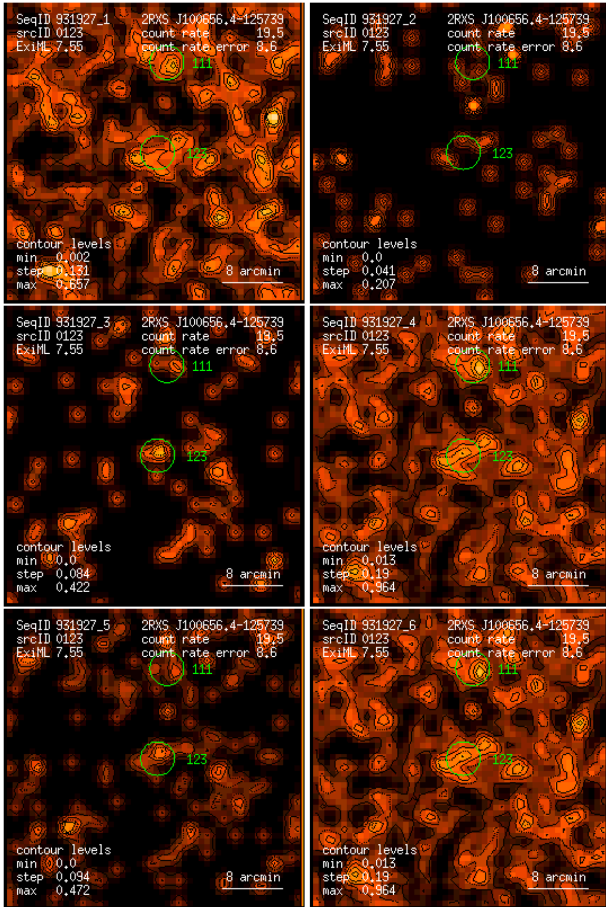
Figure 123: RASS 931927: detection 0123: band rate images, Gaussian filter: (1) PSPC channels 11 – 41, (2) 52 – 90, (3) 91 – 201, (4) 11 – 235, (5) 52 – 201, (6) 11 – 201. Broad band rates in counts/ks. Band rate contour levels in counts/ks/arcmin 2 .
