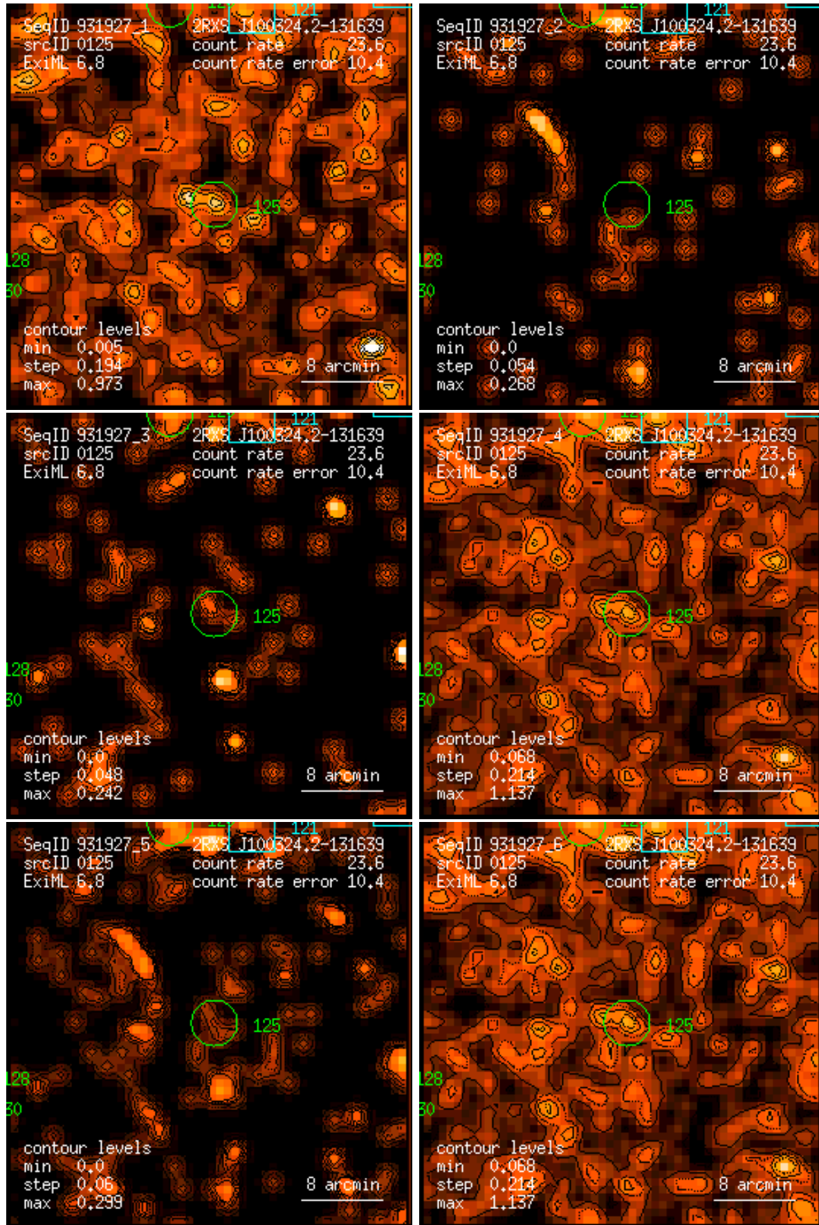
Figure 125: RASS 931927: detection 0125: band rate images, Gaussian filter: (1) PSPC channels 11 – 41, (2) 52 – 90, (3) 91 – 201, (4) 11 – 235, (5) 52 – 201, (6) 11 – 201. Broad band rates in counts/ks. Band rate contour levels in counts/ks/arcmin 2 .
