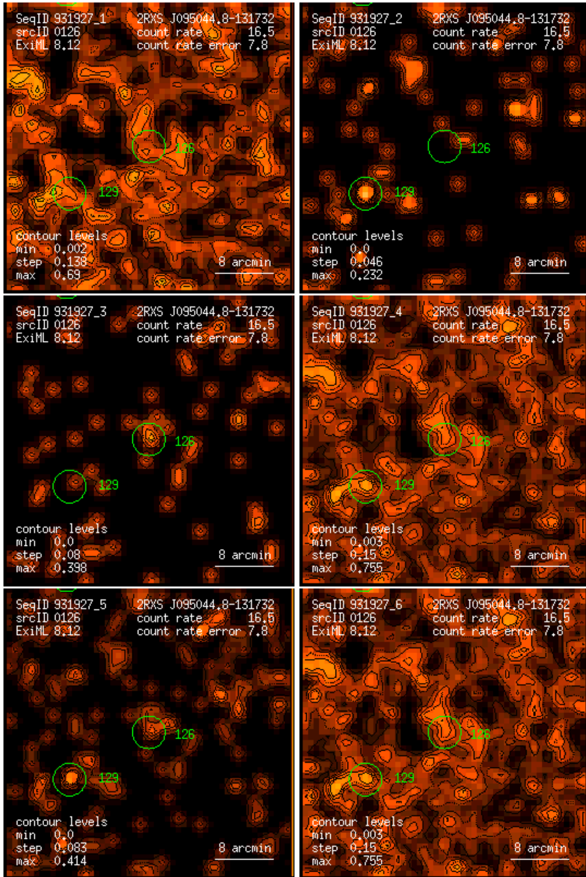
Figure 126: RASS 931927: detection 0126: band rate images, Gaussian filter: (1) PSPC channels 11 – 41, (2) 52 – 90, (3) 91 – 201, (4) 11 – 235, (5) 52 – 201, (6) 11 – 201. Broad band rates in counts/ks. Band rate contour levels in counts/ks/arcmin 2 .
