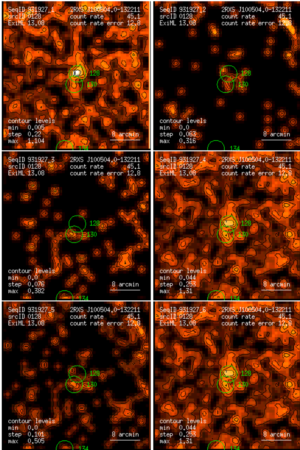
Figure 128: RASS 931927: detection 0128: band rate images, Gaussian filter: (1) PSPC channels 11 – 41, (2) 52 – 90, (3) 91 – 201, (4) 11 – 235, (5) 52 – 201, (6) 11 – 201. Broad band rates in counts/ks. Band rate contour levels in counts/ks/arcmin 2 .
