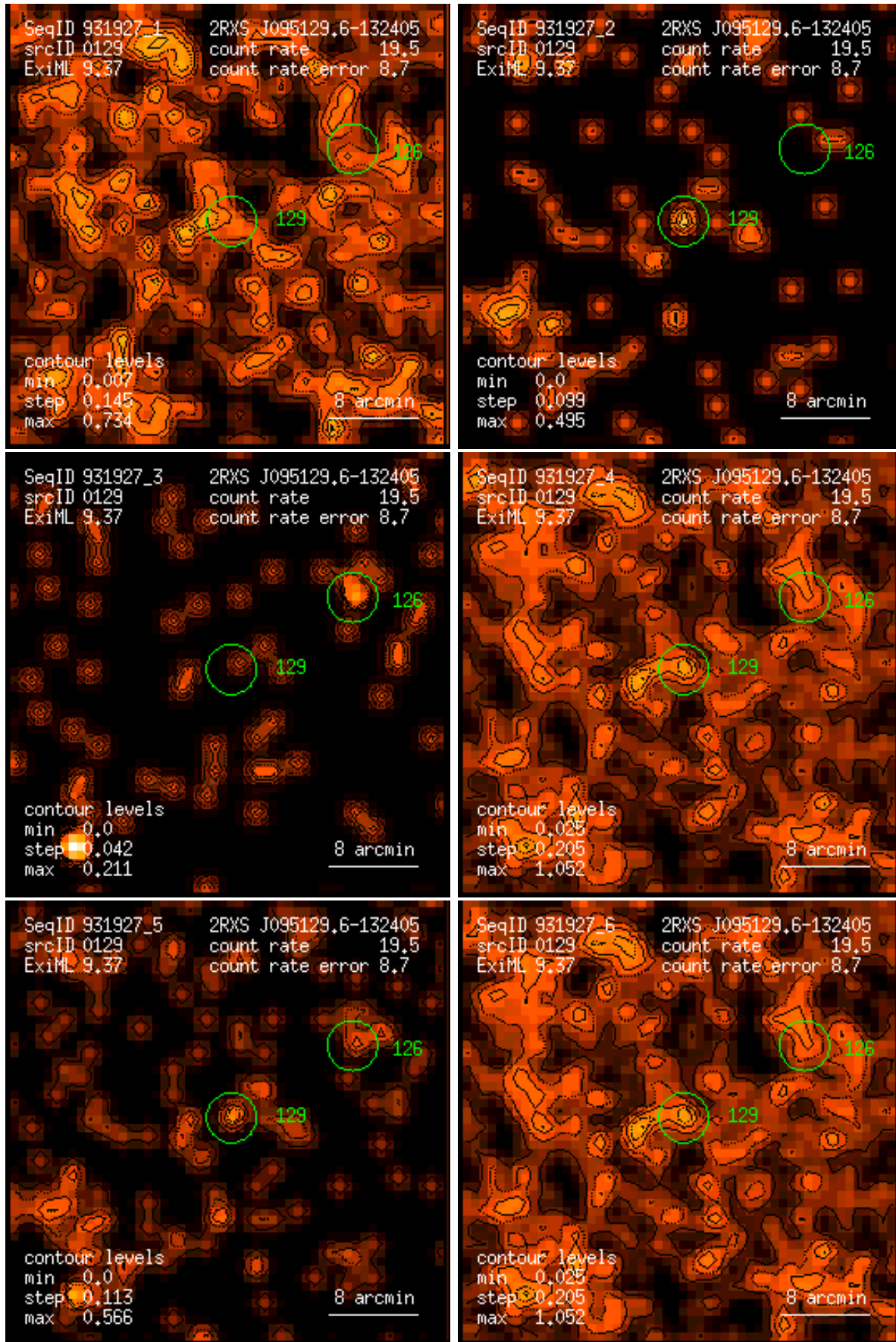
Figure 129: RASS 931927: detection 0129: band rate images, Gaussian filter: (1) PSPC channels 11 – 41, (2) 52 – 90, (3) 91 – 201, (4) 11 – 235, (5) 52 – 201, (6) 11 – 201. Broad band rates in counts/ks. Band rate contour levels in counts/ks/arcmin 2 .
