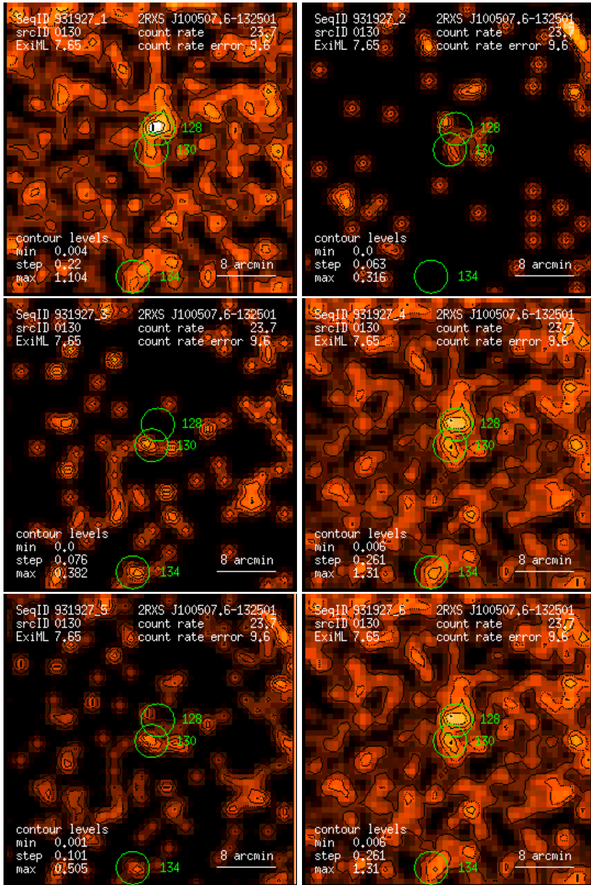
Figure 130: RASS 931927: detection 0130: band rate images, Gaussian filter: (1) PSPC channels 11 – 41, (2) 52 – 90, (3) 91 – 201, (4) 11 – 235, (5) 52 – 201, (6) 11 – 201. Broad band rates in counts/ks. Band rate contour levels in counts/ks/arcmin 2 .
