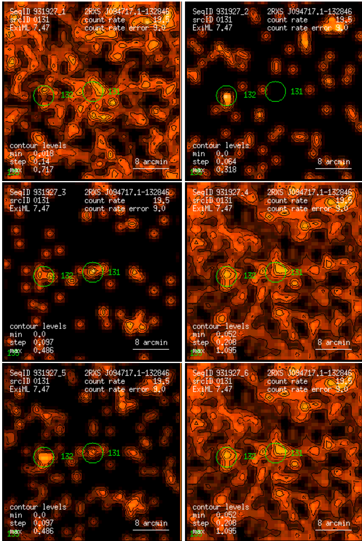
Figure 131: RASS 931927: detection 0131: band rate images, Gaussian filter: (1) PSPC channels 11 – 41, (2) 52 – 90, (3) 91 – 201, (4) 11 – 235, (5) 52 – 201, (6) 11 – 201. Broad band rates in counts/ks. Band rate contour levels in counts/ks/arcmin 2 .
