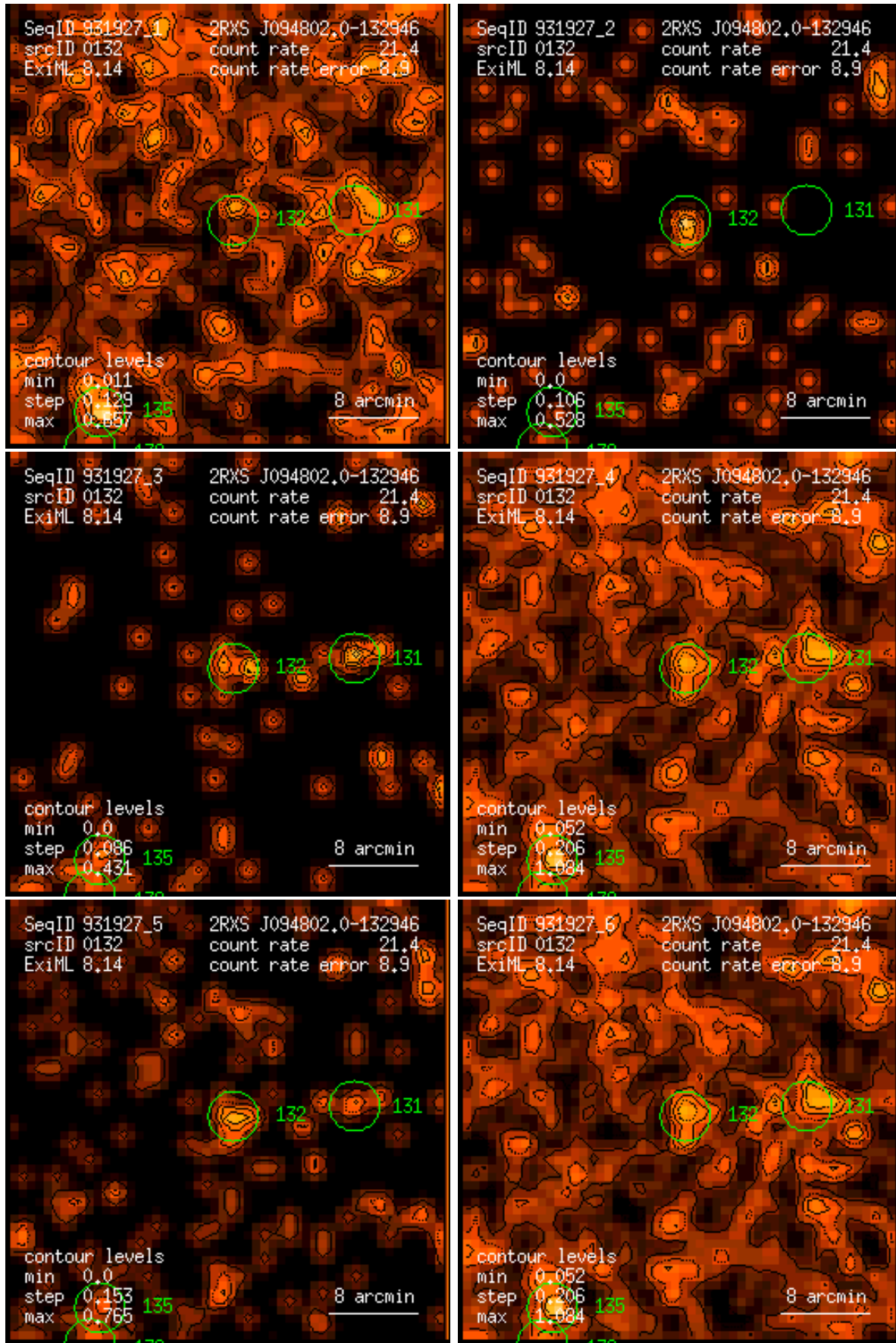
Figure 132: RASS 931927: detection 0132: band rate images, Gaussian filter: (1) PSPC channels 11 – 41, (2) 52 – 90, (3) 91 – 201, (4) 11 – 235, (5) 52 – 201, (6) 11 – 201. Broad band rates in counts/ks. Band rate contour levels in counts/ks/arcmin 2 .
