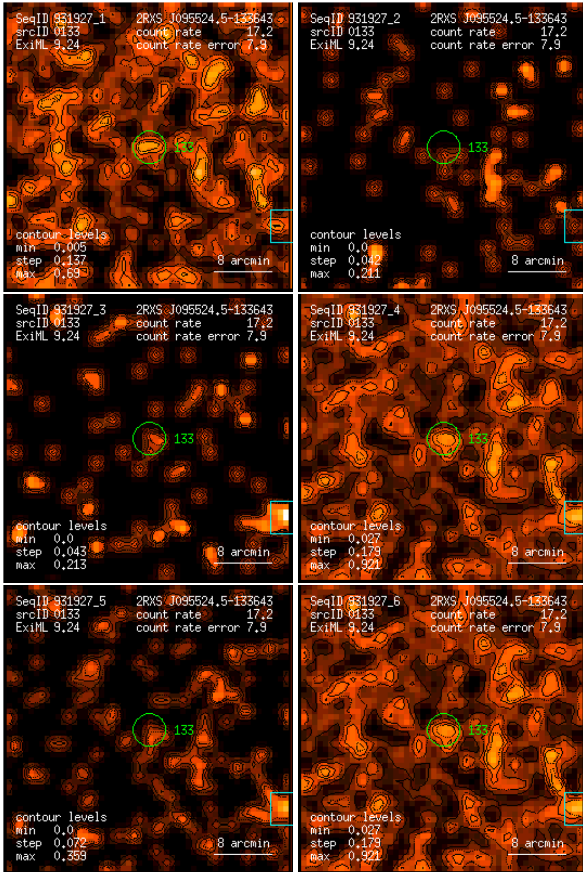
Figure 133: RASS 931927: detection 0133: band rate images, Gaussian filter: (1) PSPC channels 11 – 41, (2) 52 – 90, (3) 91 – 201, (4) 11 – 235, (5) 52 – 201, (6) 11 – 201. Broad band rates in counts/ks. Band rate contour levels in counts/ks/arcmin 2 .
