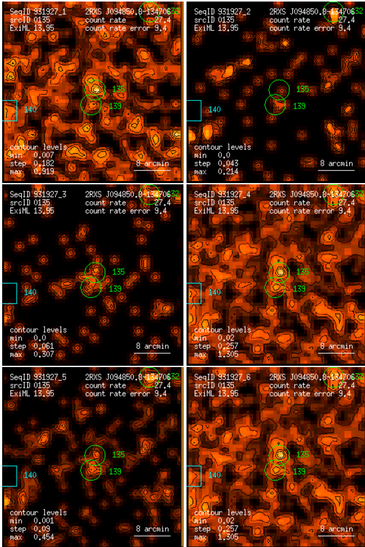
Figure 135: RASS 931927: detection 0135: band rate images, Gaussian filter: (1) PSPC channels 11 – 41, (2) 52 – 90, (3) 91 – 201, (4) 11 – 235, (5) 52 – 201, (6) 11 – 201. Broad band rates in counts/ks. Band rate contour levels in counts/ks/arcmin 2 .
