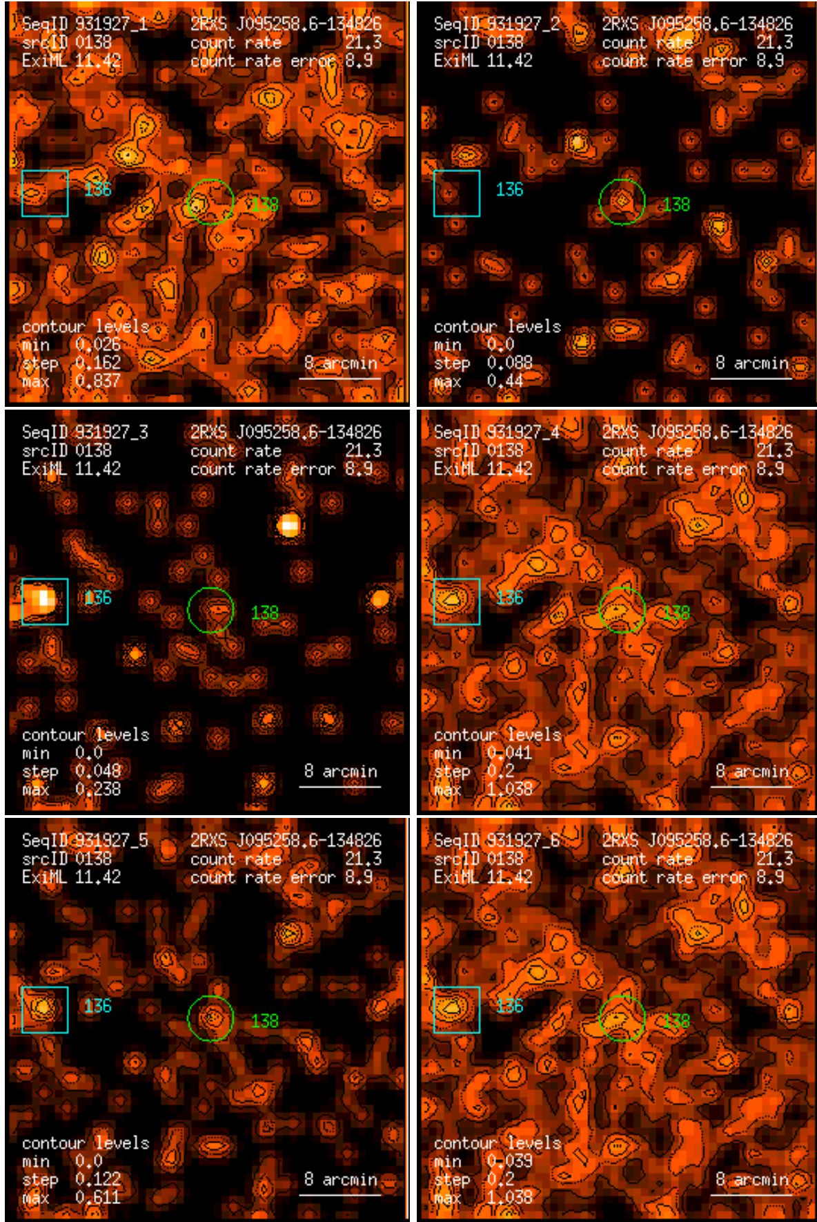
Figure 138: RASS 931927: detection 0138: band rate images, Gaussian filter: (1) PSPC channels 11 – 41, (2) 52 – 90, (3) 91 – 201, (4) 11 – 235, (5) 52 – 201, (6) 11 – 201. Broad band rates in counts/ks. Band rate contour levels in counts/ks/arcmin 2 .
