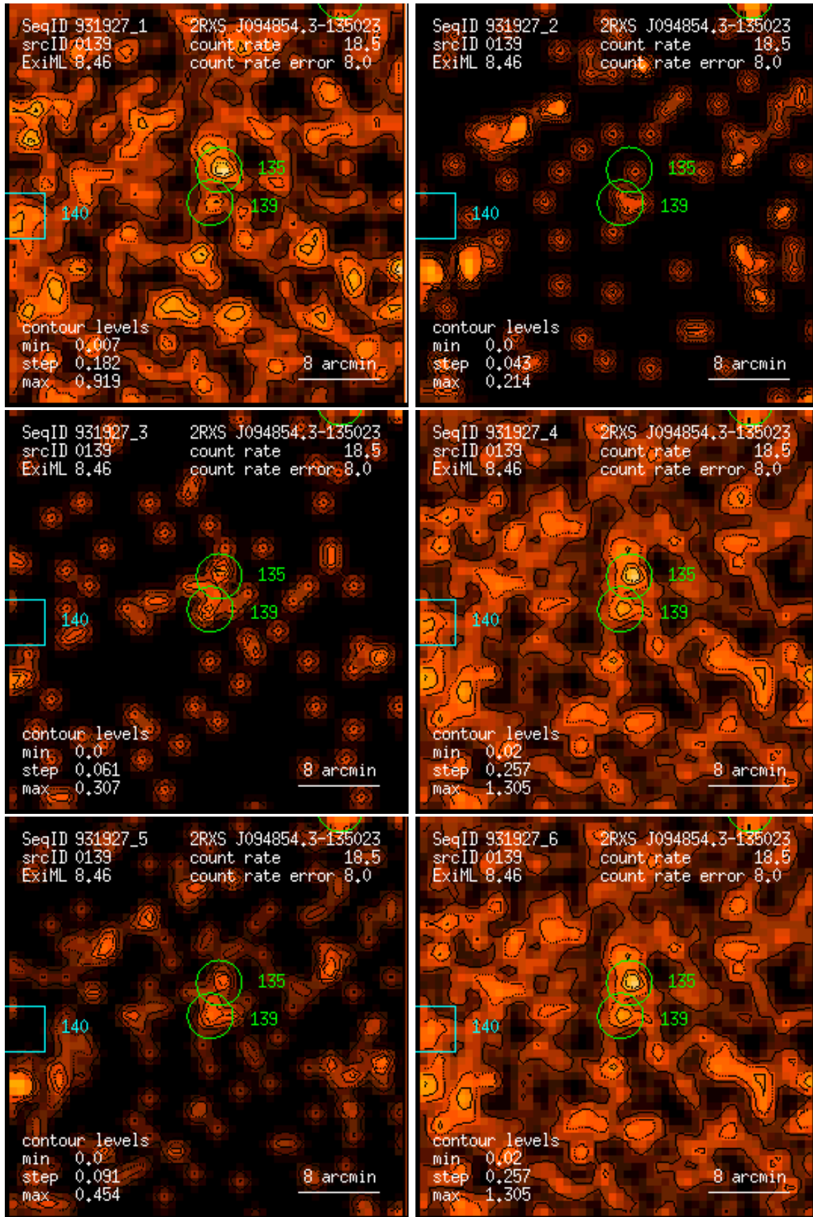
Figure 139: RASS 931927: detection 0139: band rate images, Gaussian filter: (1) PSPC channels 11 – 41, (2) 52 – 90, (3) 91 – 201, (4) 11 – 235, (5) 52 – 201, (6) 11 – 201. Broad band rates in counts/ks. Band rate contour levels in counts/ks/arcmin 2 .
