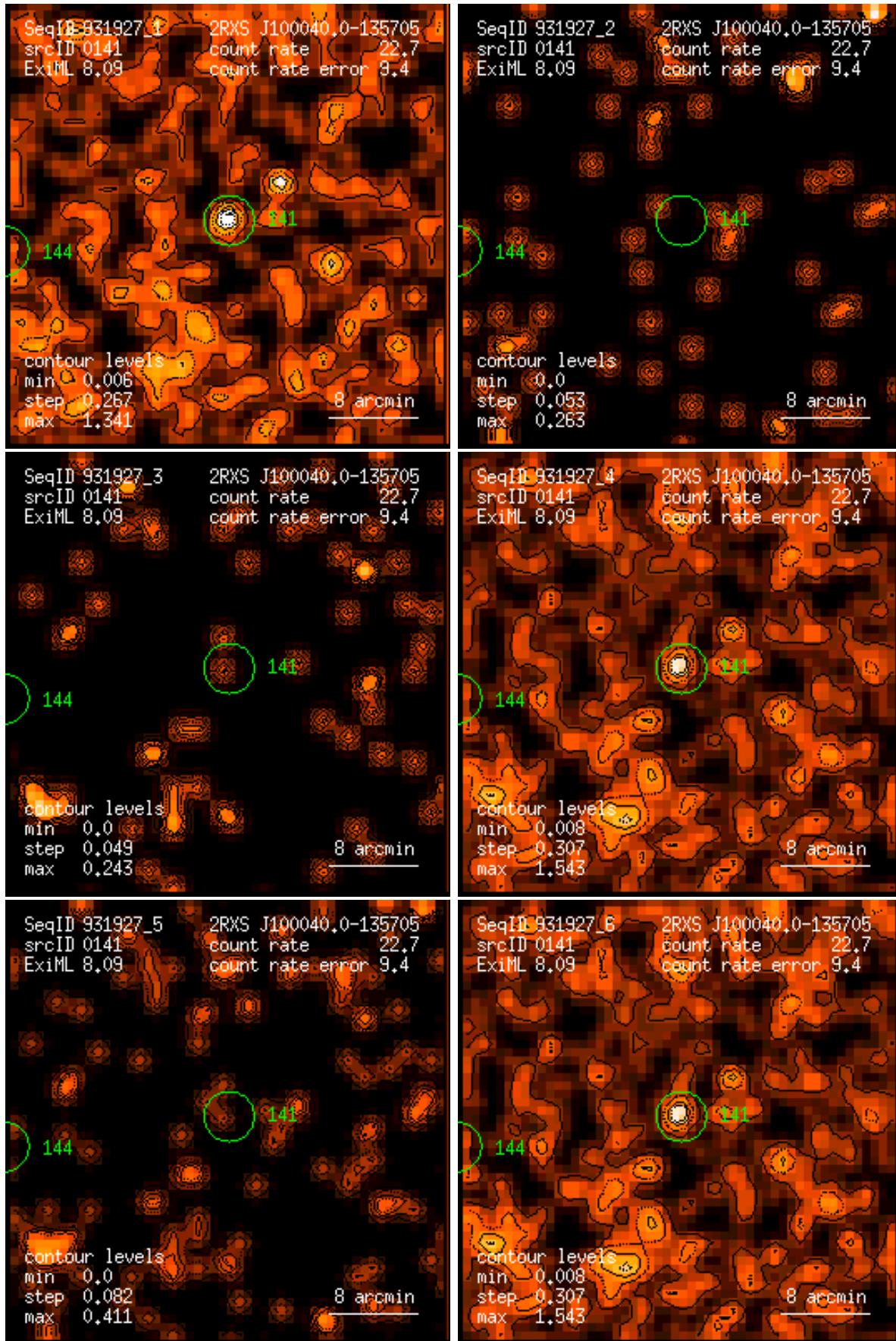
Figure 141: RASS 931927: detection 0141: band rate images, Gaussian filter: (1) PSPC channels 11 – 41, (2) 52 – 90, (3) 91 – 201, (4) 11 – 235, (5) 52 – 201, (6) 11 – 201. Broad band rates in counts/ks. Band rate contour levels in counts/ks/arcmin 2 .
