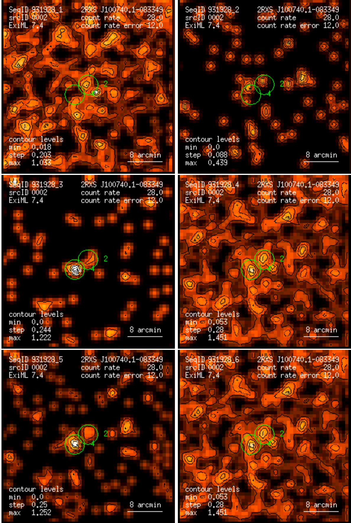
Figure 2: RASS 931928: detection 0002: band rate images, Gaussian filter: (1) PSPC channels 11 – 41, (2) 52 – 90, (3) 91 – 201, (4) 11 – 235, (5) 52 – 201, (6) 11 – 201. Broad band rates in counts/ks. Band rate contour levels in counts/ks/arcmin 2 .
