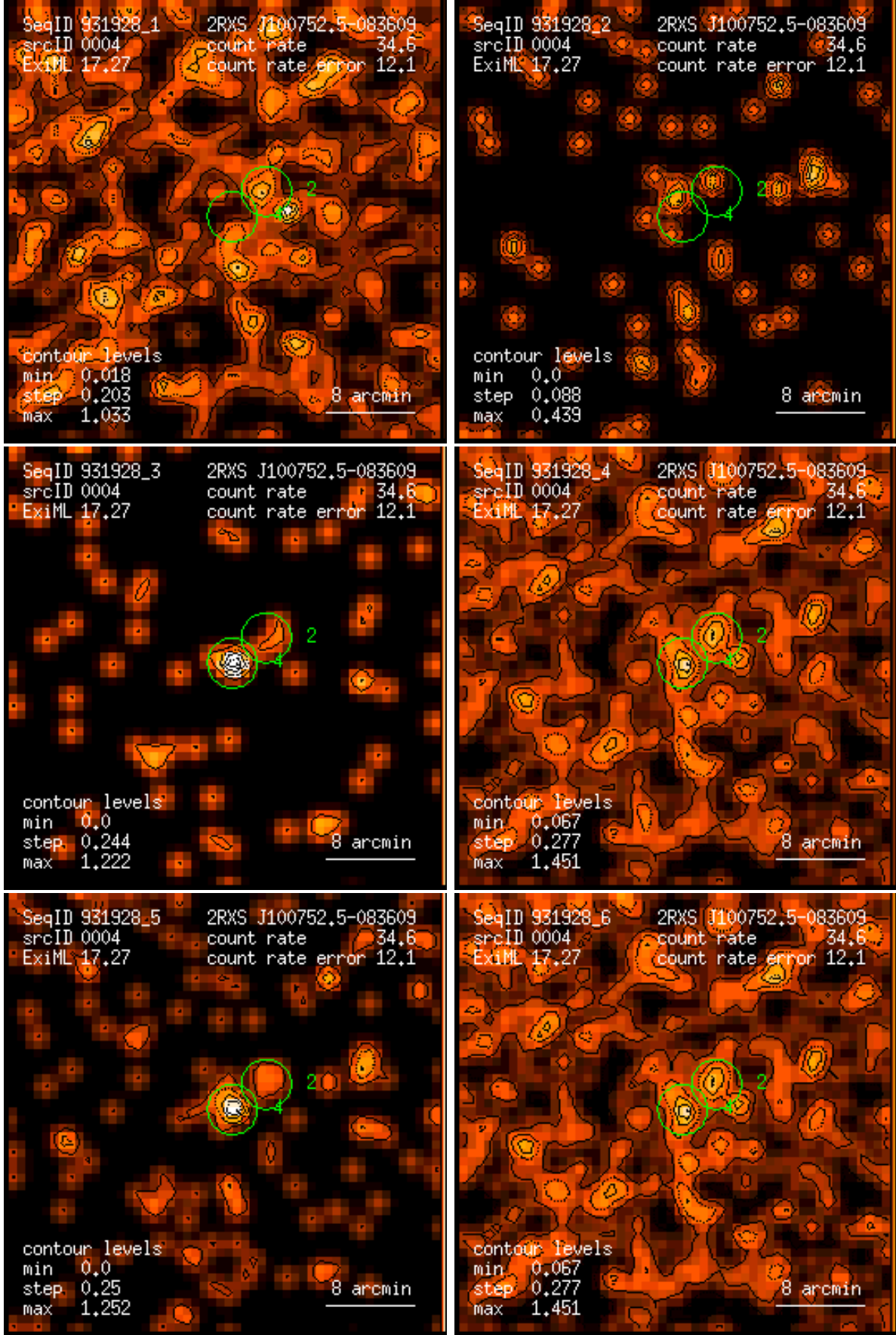
Figure 4: RASS 931928: detection 0004: band rate images, Gaussian filter: (1) PSPC channels 11 – 41, (2) 52 – 90, (3) 91 – 201, (4) 11 – 235, (5) 52 – 201, (6) 11 – 201. Broad band rates in counts/ks. Band rate contour levels in counts/ks/arcmin 2 .
