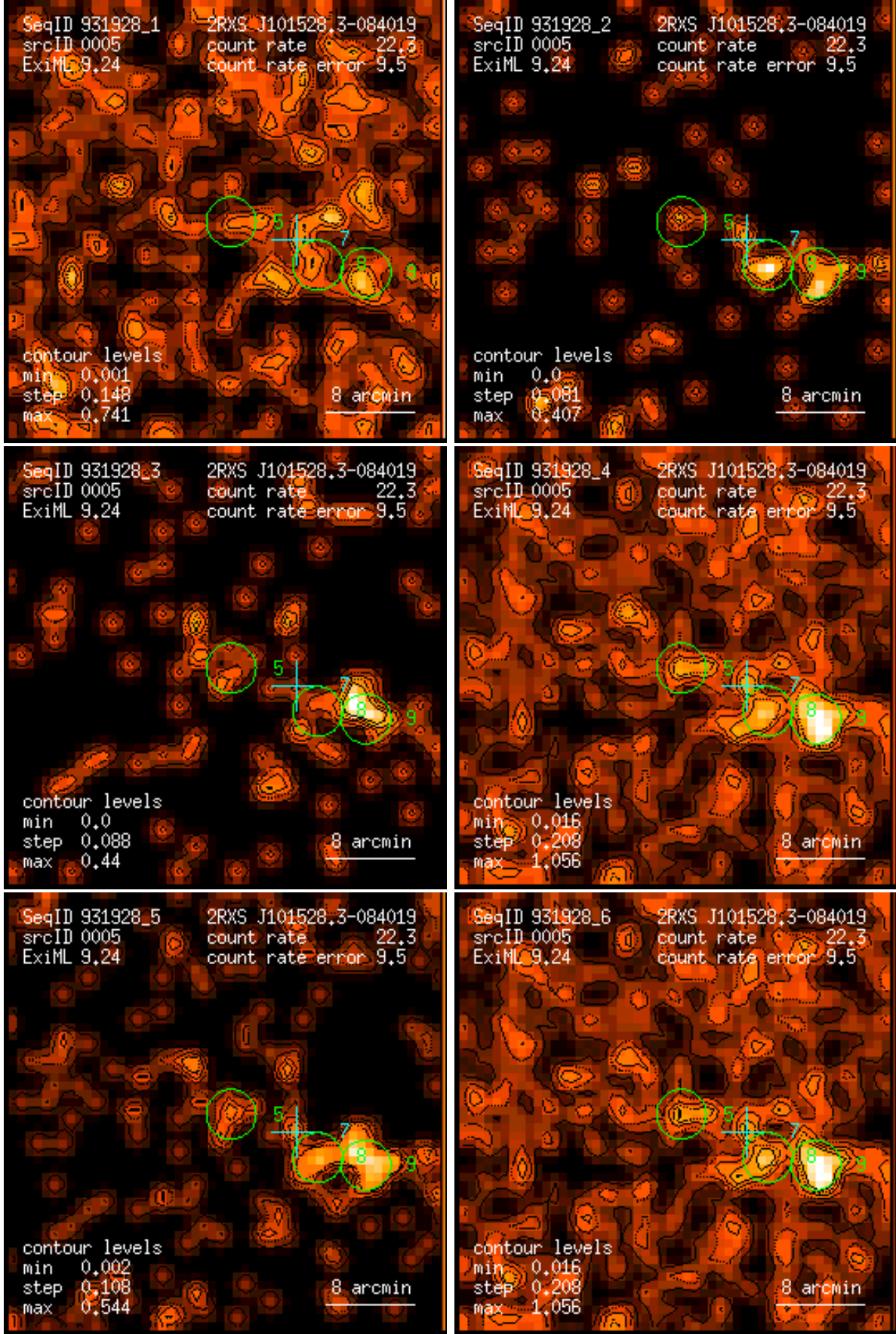
Figure 5: RASS 931928: detection 0005: band rate images, Gaussian filter: (1) PSPC channels 11 – 41, (2) 52 – 90, (3) 91 – 201, (4) 11 – 235, (5) 52 – 201, (6) 11 – 201. Broad band rates in counts/ks. Band rate contour levels in counts/ks/arcmin 2 .
