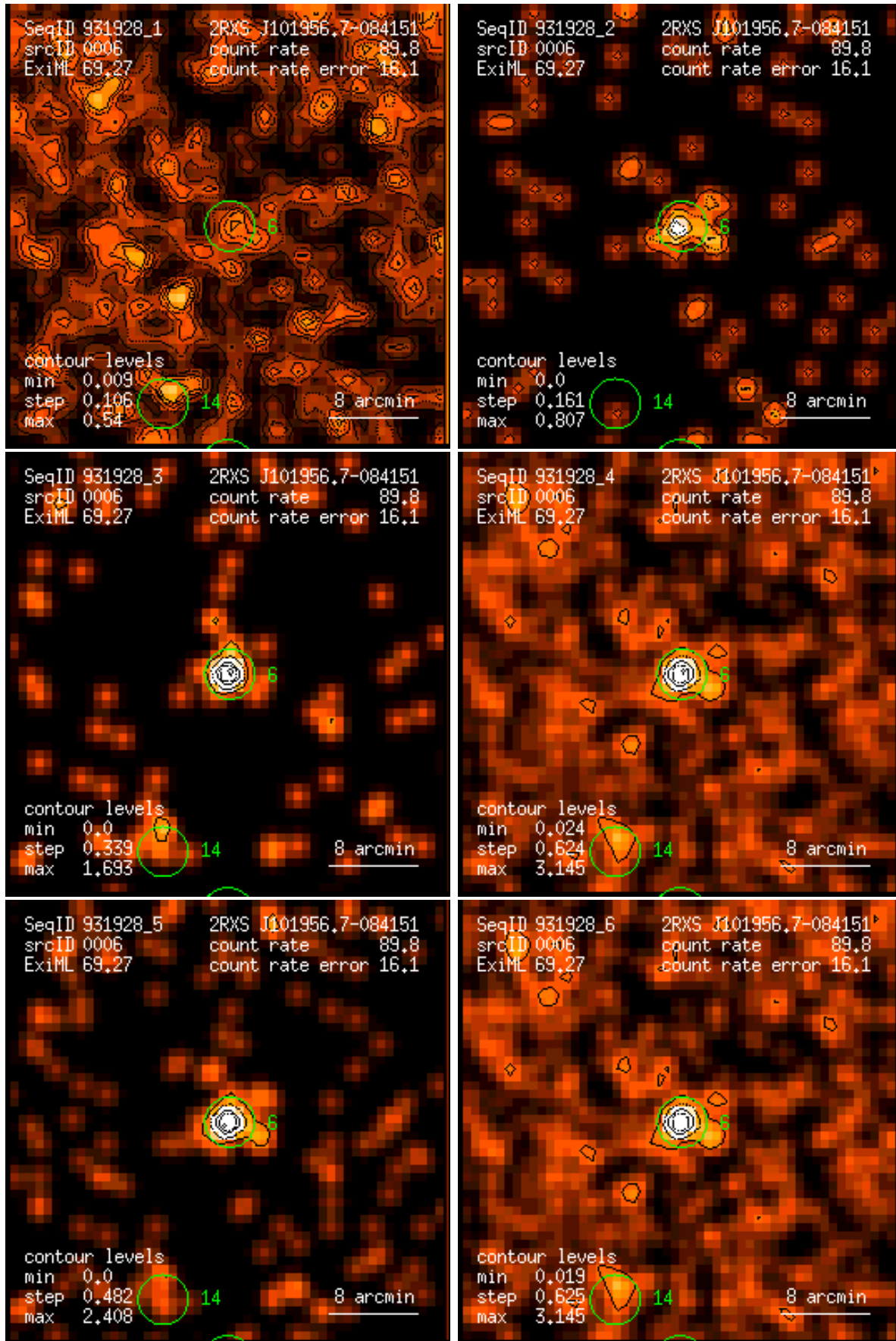
Figure 6: RASS 931928: detection 0006: band rate images, Gaussian filter: (1) PSPC channels 11 – 41, (2) 52 – 90, (3) 91 – 201, (4) 11 – 235, (5) 52 – 201, (6) 11 – 201. Broad band rates in counts/ks. Band rate contour levels in counts/ks/arcmin 2 .
