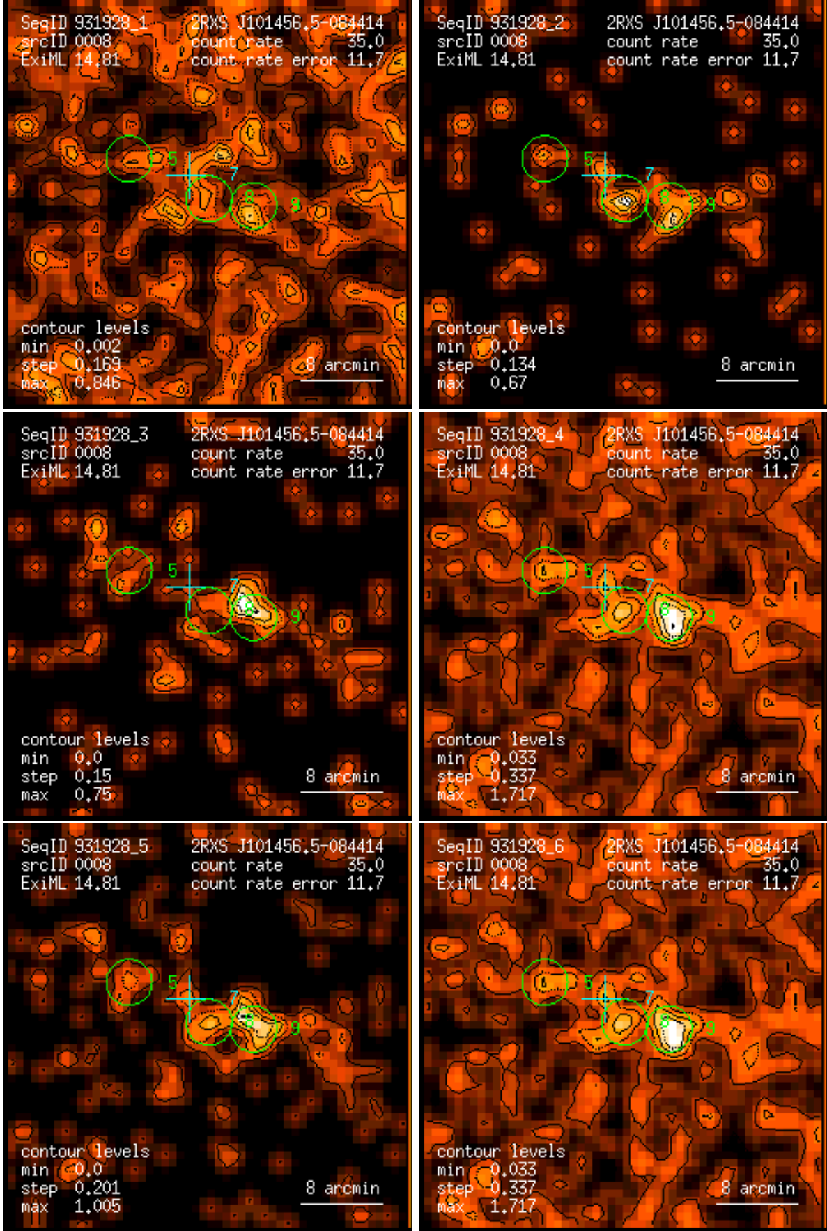
Figure 8: RASS 931928: detection 0008: band rate images, Gaussian filter: (1) PSPC channels 11 – 41, (2) 52 – 90, (3) 91 – 201, (4) 11 – 235, (5) 52 – 201, (6) 11 – 201. Broad band rates in counts/ks. Band rate contour levels in counts/ks/arcmin 2 .
