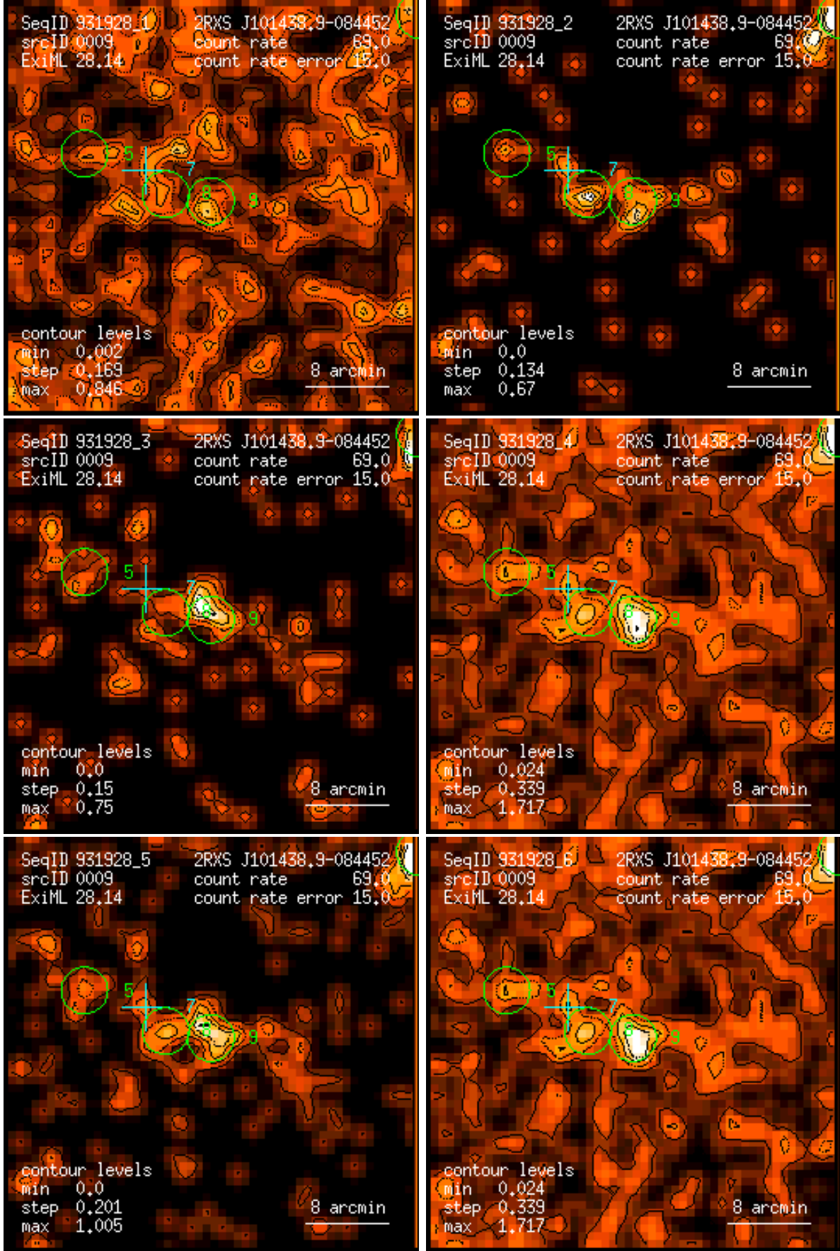
Figure 9: RASS 931928: detection 0009: band rate images, Gaussian filter: (1) PSPC channels 11 – 41, (2) 52 – 90, (3) 91 – 201, (4) 11 – 235, (5) 52 – 201, (6) 11 – 201. Broad band rates in counts/ks. Band rate contour levels in counts/ks/arcmin 2 .
