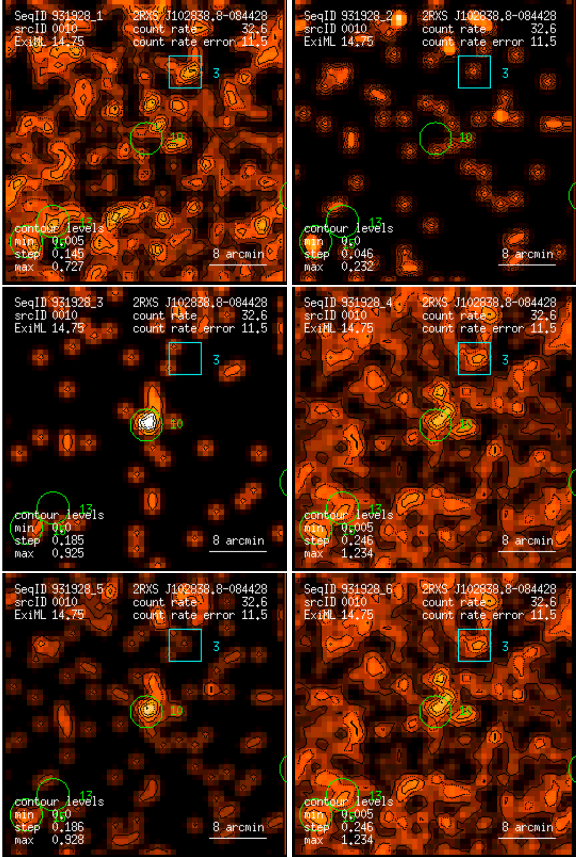
Figure 10: RASS 931928: detection 0010: band rate images, Gaussian filter: (1) PSPC channels 11 – 41, (2) 52 – 90, (3) 91 – 201, (4) 11 – 235, (5) 52 – 201, (6) 11 – 201. Broad band rates in counts/ks. Band rate contour levels in counts/ks/arcmin 2 .
