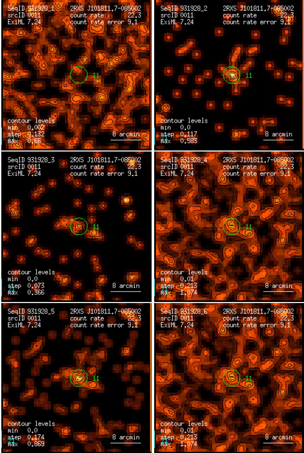
Figure 11: RASS 931928: detection 0011: band rate images, Gaussian filter: (1) PSPC channels 11 – 41, (2) 52 – 90, (3) 91 – 201, (4) 11 – 235, (5) 52 – 201, (6) 11 – 201. Broad band rates in counts/ks. Band rate contour levels in counts/ks/arcmin 2 .
