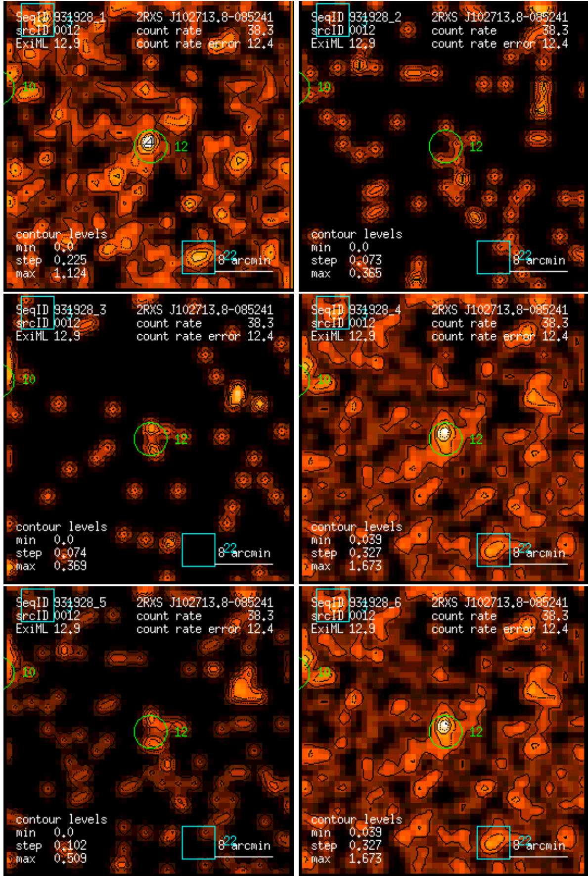
Figure 12: RASS 931928: detection 0012: band rate images, Gaussian filter: (1) PSPC channels 11 – 41, (2) 52 – 90, (3) 91 – 201, (4) 11 – 235, (5) 52 – 201, (6) 11 – 201. Broad band rates in counts/ks. Band rate contour levels in counts/ks/arcmin 2 .
