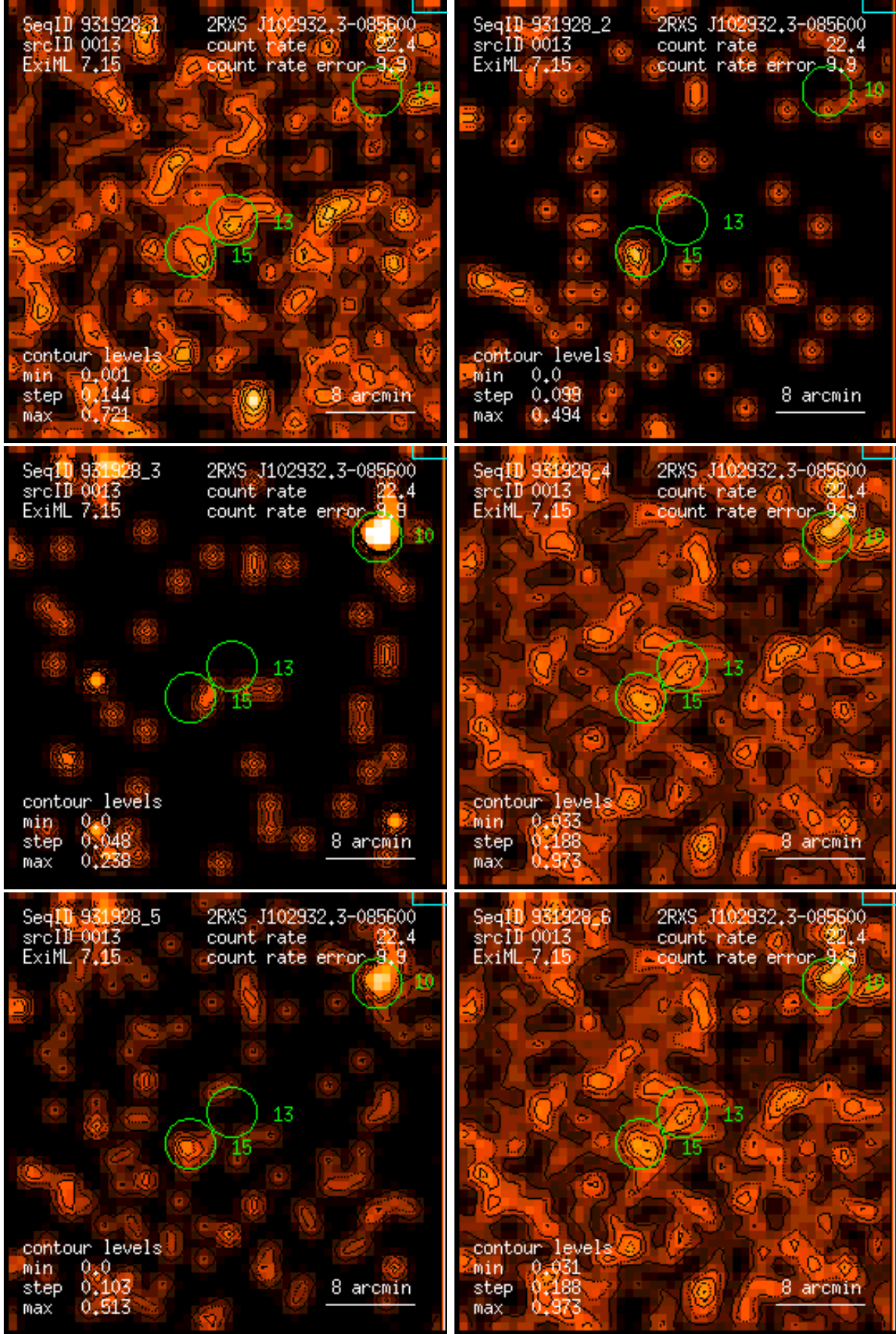
Figure 13: RASS 931928: detection 0013: band rate images, Gaussian filter: (1) PSPC channels 11 – 41, (2) 52 – 90, (3) 91 – 201, (4) 11 – 235, (5) 52 – 201, (6) 11 – 201. Broad band rates in counts/ks. Band rate contour levels in counts/ks/arcmin 2 .
