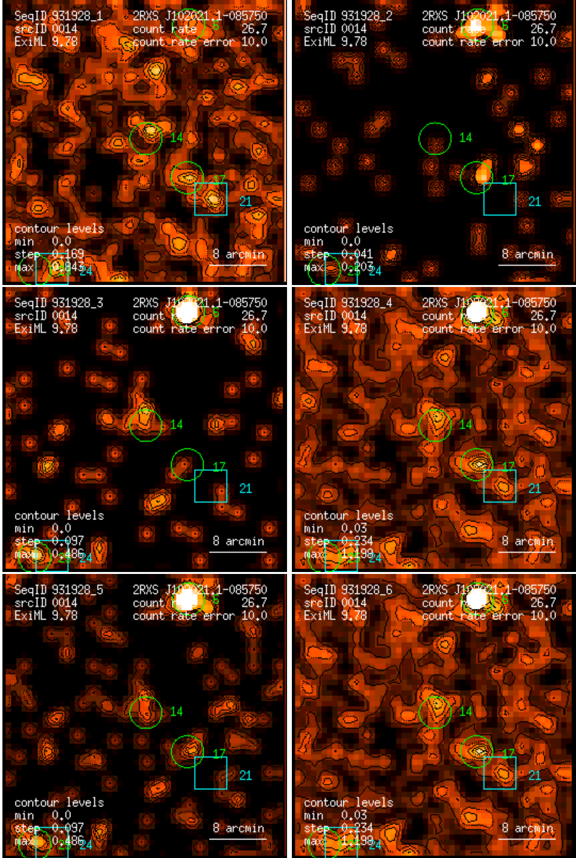
Figure 14: RASS 931928: detection 0014: band rate images, Gaussian filter: (1) PSPC channels 11 – 41, (2) 52 – 90, (3) 91 – 201, (4) 11 – 235, (5) 52 – 201, (6) 11 – 201. Broad band rates in counts/ks. Band rate contour levels in counts/ks/arcmin 2 .
