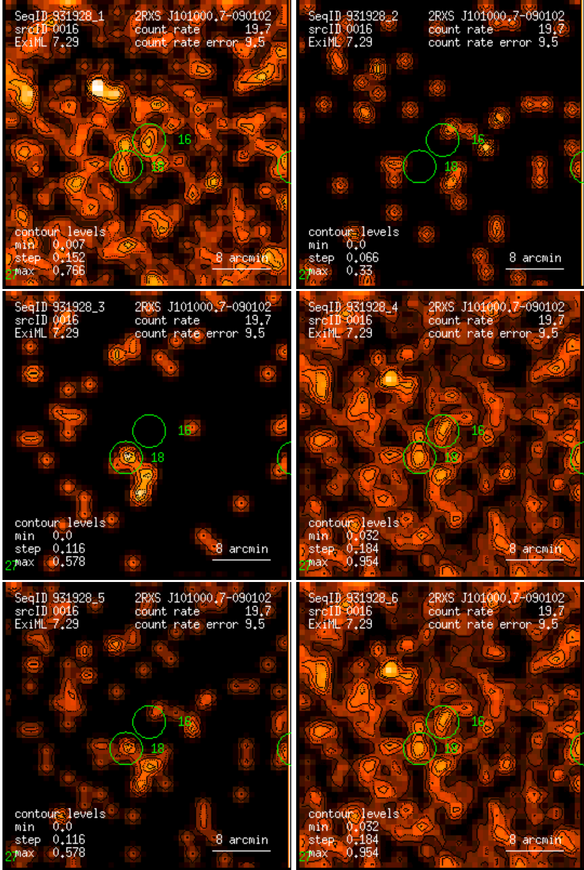
Figure 16: RASS 931928: detection 0016: band rate images, Gaussian filter: (1) PSPC channels 11 – 41, (2) 52 – 90, (3) 91 – 201, (4) 11 – 235, (5) 52 – 201, (6) 11 – 201. Broad band rates in counts/ks. Band rate contour levels in counts/ks/arcmin 2 .
