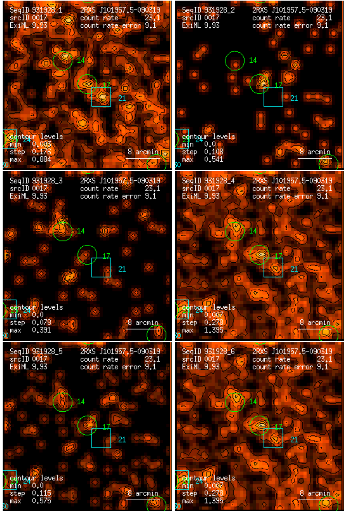
Figure 17: RASS 931928: detection 0017: band rate images, Gaussian filter: (1) PSPC channels 11 – 41, (2) 52 – 90, (3) 91 – 201, (4) 11 – 235, (5) 52 – 201, (6) 11 – 201. Broad band rates in counts/ks. Band rate contour levels in counts/ks/arcmin 2 .
