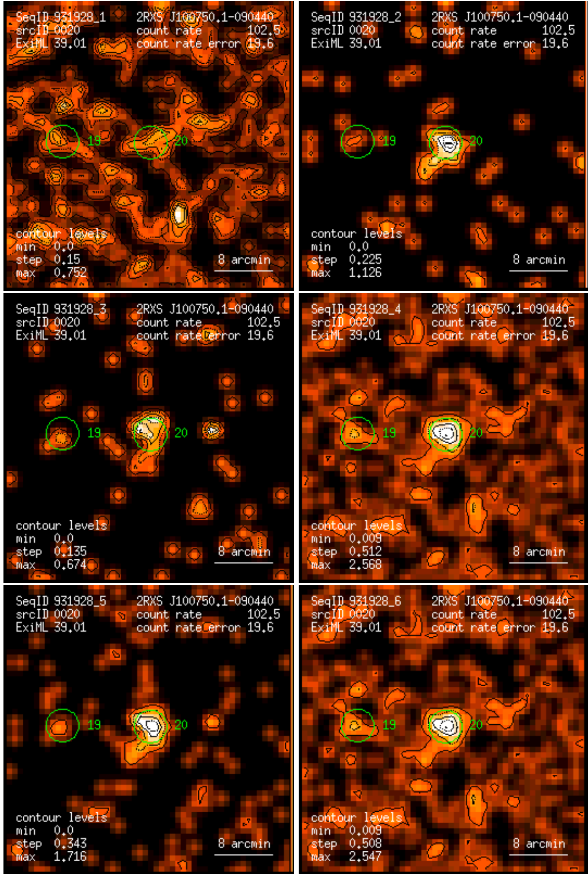
Figure 20: RASS 931928: detection 0020: band rate images, Gaussian filter: (1) PSPC channels 11 – 41, (2) 52 – 90, (3) 91 – 201, (4) 11 – 235, (5) 52 – 201, (6) 11 – 201. Broad band rates in counts/ks. Band rate contour levels in counts/ks/arcmin 2 .
