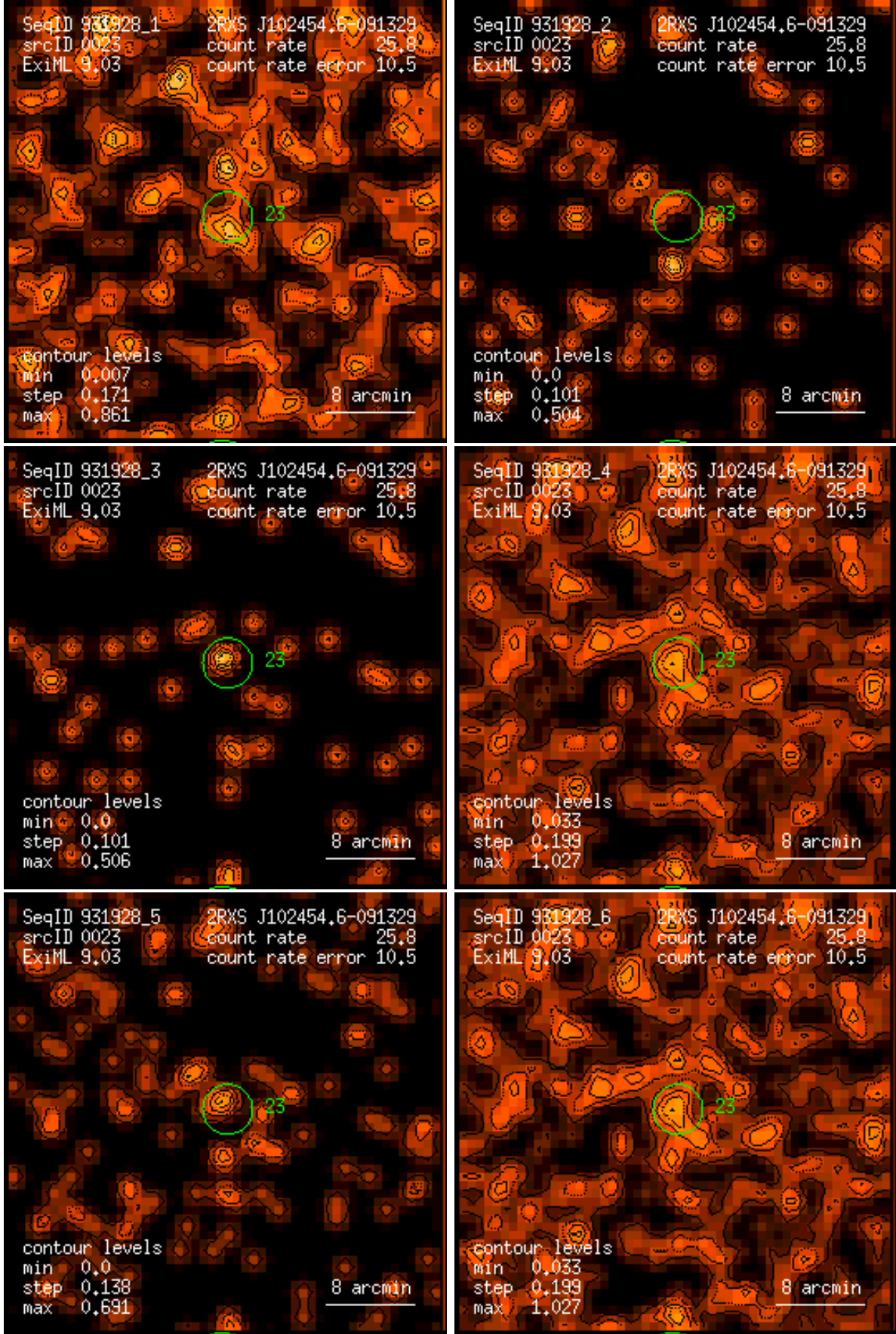
Figure 23: RASS 931928: detection 0023: band rate images, Gaussian filter: (1) PSPC channels 11 – 41, (2) 52 – 90, (3) 91 – 201, (4) 11 – 235, (5) 52 – 201, (6) 11 – 201. Broad band rates in counts/ks. Band rate contour levels in counts/ks/arcmin 2 .
