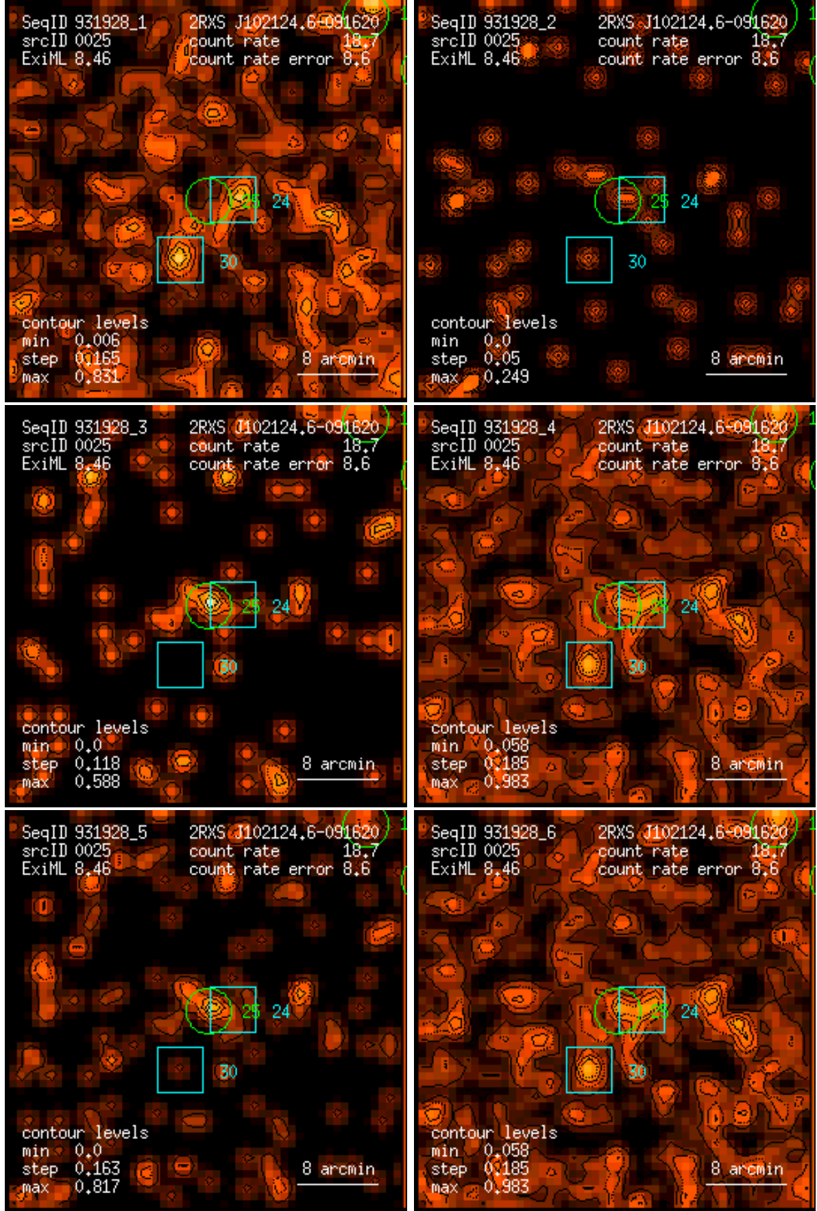
Figure 25: RASS 931928: detection 0025: band rate images, Gaussian filter: (1) PSPC channels 11 – 41, (2) 52 – 90, (3) 91 – 201, (4) 11 – 235, (5) 52 – 201, (6) 11 – 201. Broad band rates in counts/ks. Band rate contour levels in counts/ks/arcmin 2 .
