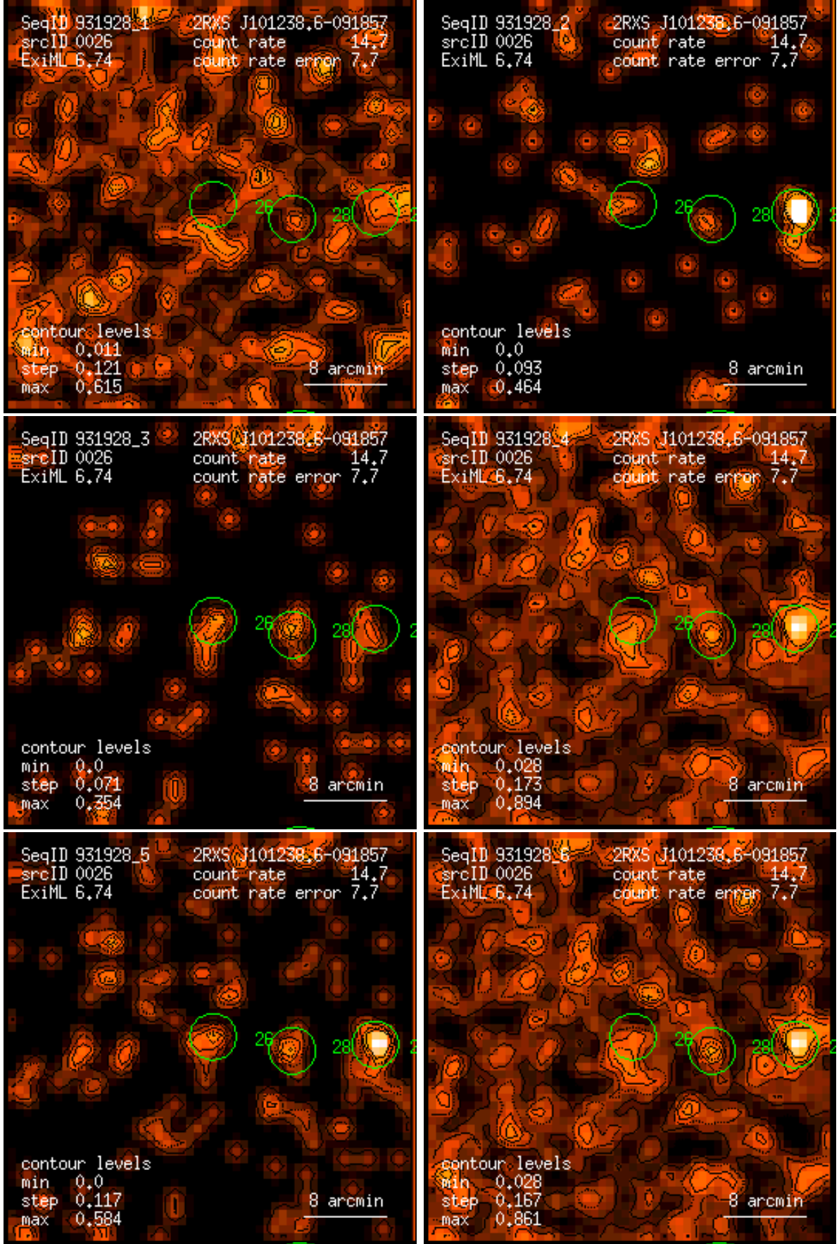
Figure 26: RASS 931928: detection 0026: band rate images, Gaussian filter: (1) PSPC channels 11 – 41, (2) 52 – 90, (3) 91 – 201, (4) 11 – 235, (5) 52 – 201, (6) 11 – 201. Broad band rates in counts/ks. Band rate contour levels in counts/ks/arcmin 2 .
