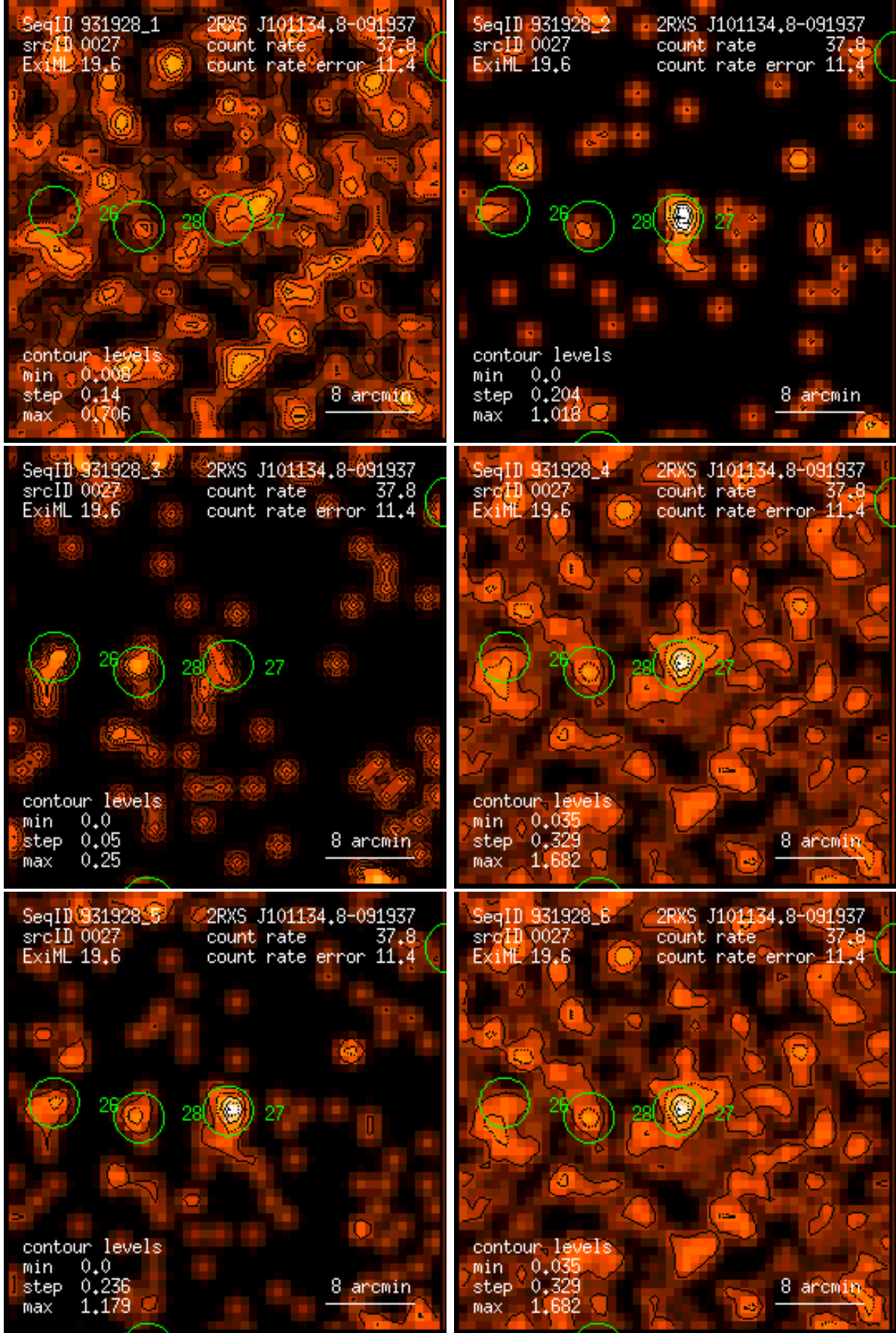
Figure 27: RASS 931928: detection 0027: band rate images, Gaussian filter: (1) PSPC channels 11 – 41, (2) 52 – 90, (3) 91 – 201, (4) 11 – 235, (5) 52 – 201, (6) 11 – 201. Broad band rates in counts/ks. Band rate contour levels in counts/ks/arcmin 2 .
