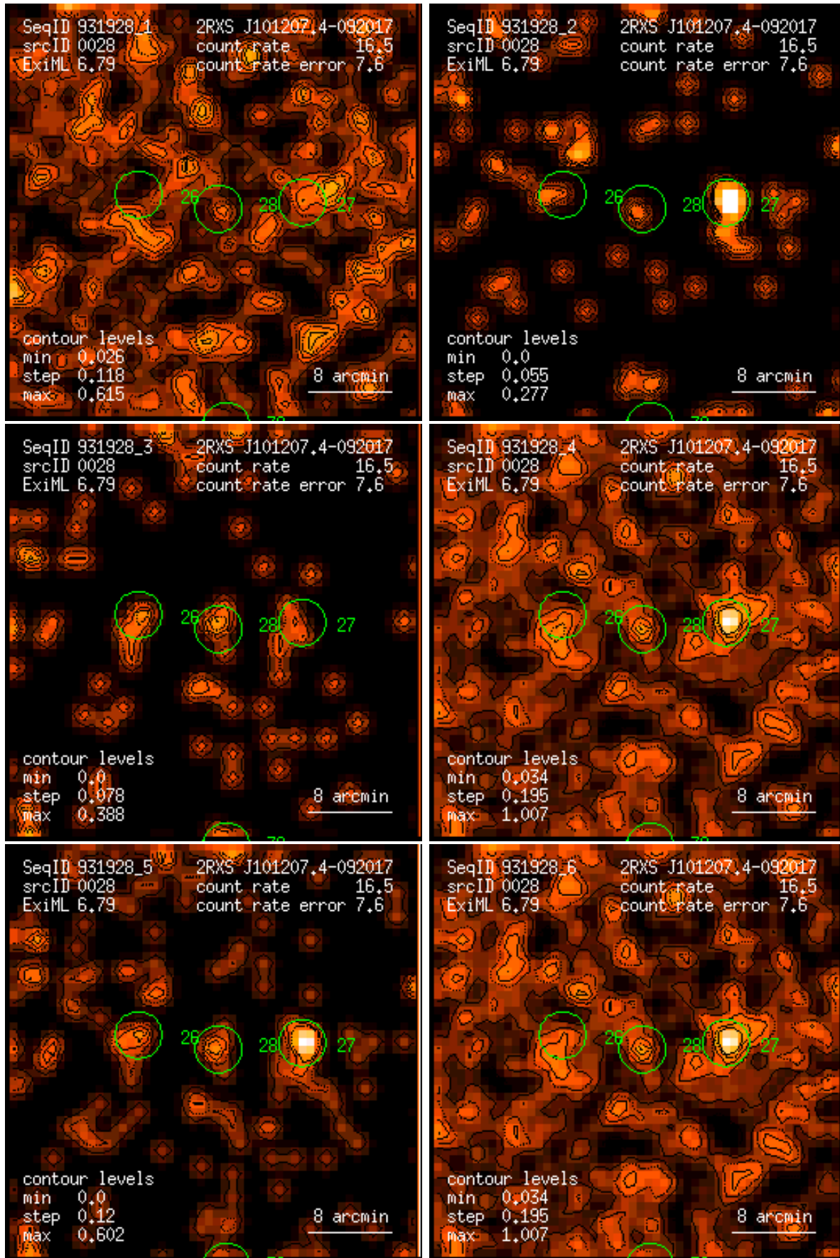
Figure 28: RASS 931928: detection 0028: band rate images, Gaussian filter: (1) PSPC channels 11 – 41, (2) 52 – 90, (3) 91 – 201, (4) 11 – 235, (5) 52 – 201, (6) 11 – 201. Broad band rates in counts/ks. Band rate contour levels in counts/ks/arcmin 2 .
