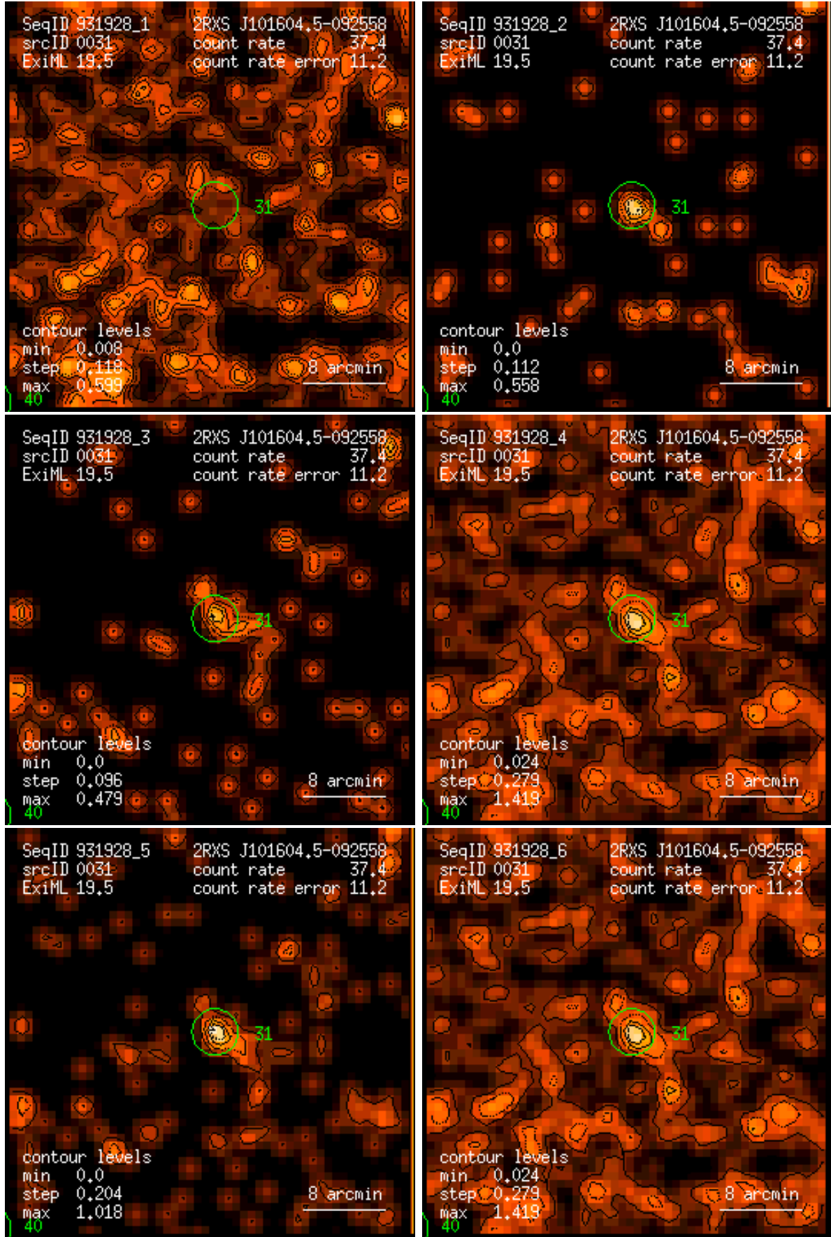
Figure 31: RASS 931928: detection 0031: band rate images, Gaussian filter: (1) PSPC channels 11 – 41, (2) 52 – 90, (3) 91 – 201, (4) 11 – 235, (5) 52 – 201, (6) 11 – 201. Broad band rates in counts/ks. Band rate contour levels in counts/ks/arcmin 2 .
