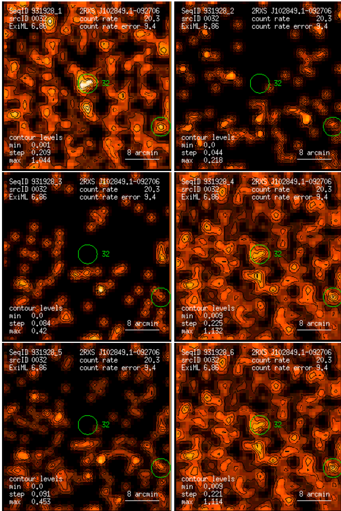
Figure 32: RASS 931928: detection 0032: band rate images, Gaussian filter: (1) PSPC channels 11 – 41, (2) 52 – 90, (3) 91 – 201, (4) 11 – 235, (5) 52 – 201, (6) 11 – 201. Broad band rates in counts/ks. Band rate contour levels in counts/ks/arcmin 2 .
