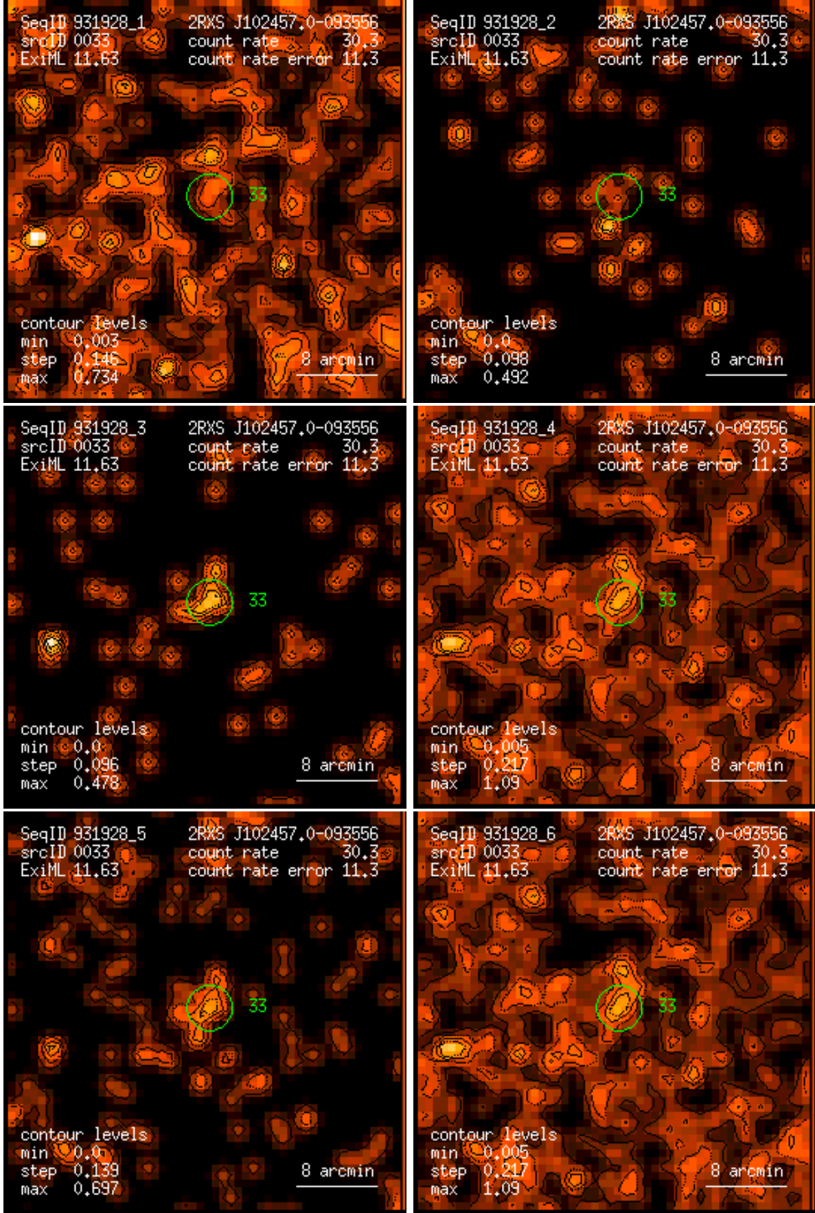
Figure 33: RASS 931928: detection 0033: band rate images, Gaussian filter: (1) PSPC channels 11 – 41, (2) 52 – 90, (3) 91 – 201, (4) 11 – 235, (5) 52 – 201, (6) 11 – 201. Broad band rates in counts/ks. Band rate contour levels in counts/ks/arcmin 2 .
