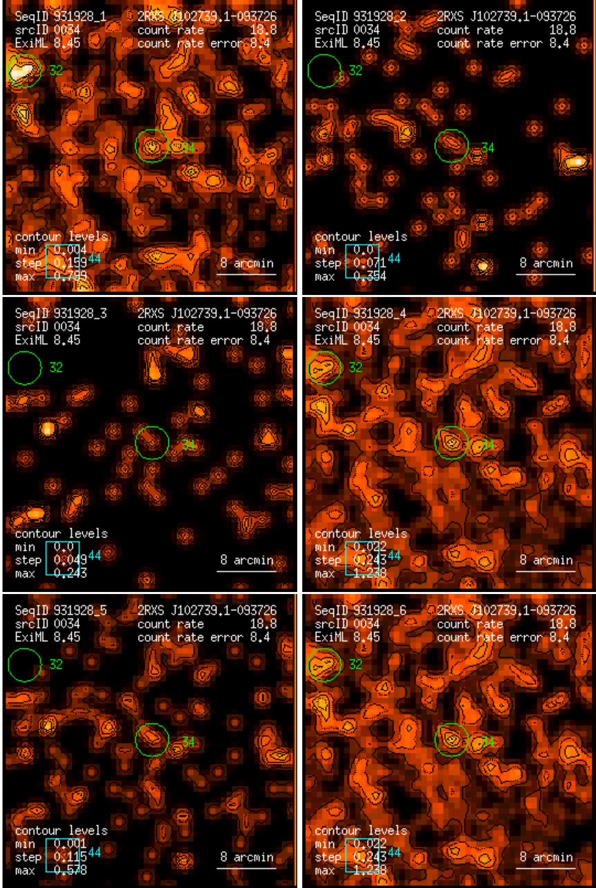
Figure 34: RASS 931928: detection 0034: band rate images, Gaussian filter: (1) PSPC channels 11 – 41, (2) 52 – 90, (3) 91 – 201, (4) 11 – 235, (5) 52 – 201, (6) 11 – 201. Broad band rates in counts/ks. Band rate contour levels in counts/ks/arcmin 2 .
