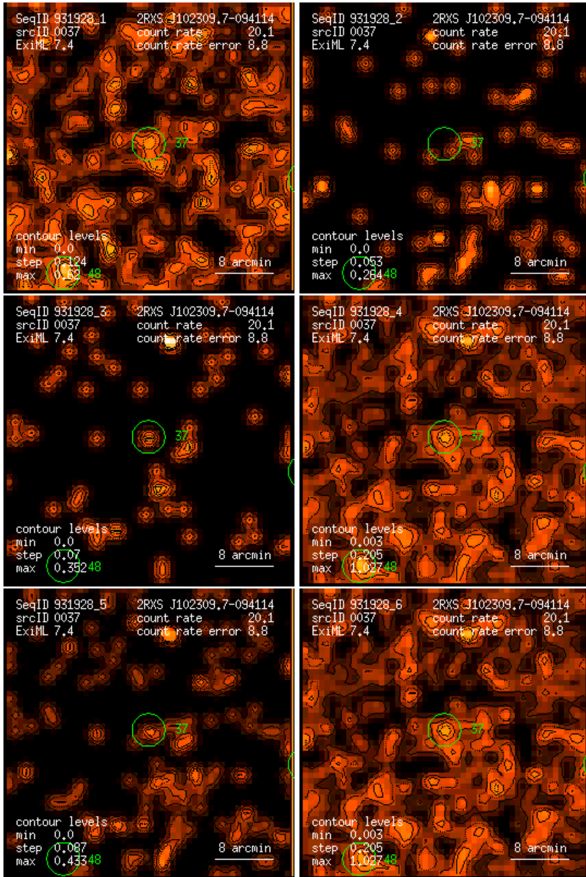
Figure 37: RASS 931928: detection 0037: band rate images, Gaussian filter: (1) PSPC channels 11 – 41, (2) 52 – 90, (3) 91 – 201, (4) 11 – 235, (5) 52 – 201, (6) 11 – 201. Broad band rates in counts/ks. Band rate contour levels in counts/ks/arcmin 2 .
