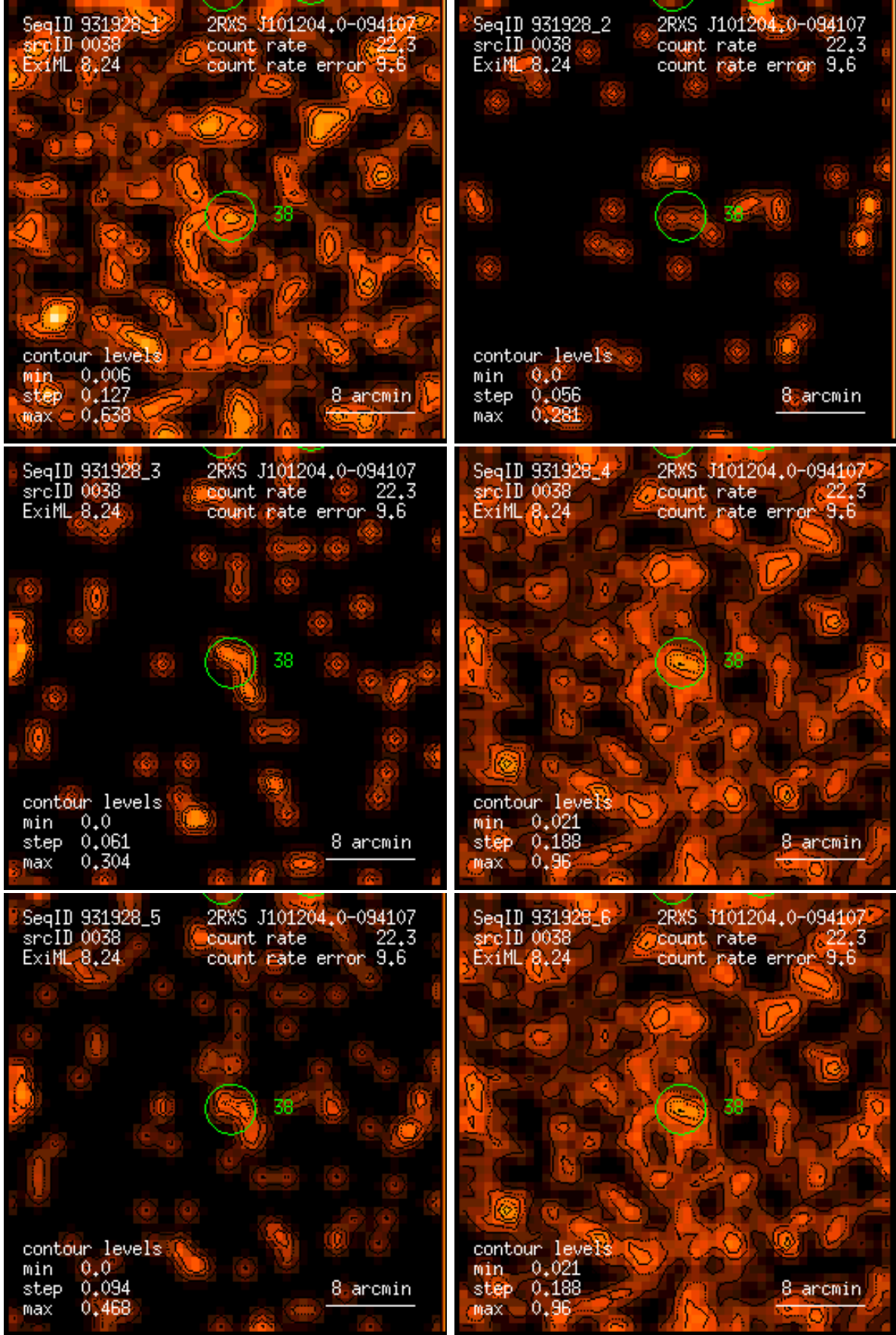
Figure 38: RASS 931928: detection 0038: band rate images, Gaussian filter: (1) PSPC channels 11 – 41, (2) 52 – 90, (3) 91 – 201, (4) 11 – 235, (5) 52 – 201, (6) 11 – 201. Broad band rates in counts/ks. Band rate contour levels in counts/ks/arcmin 2 .
