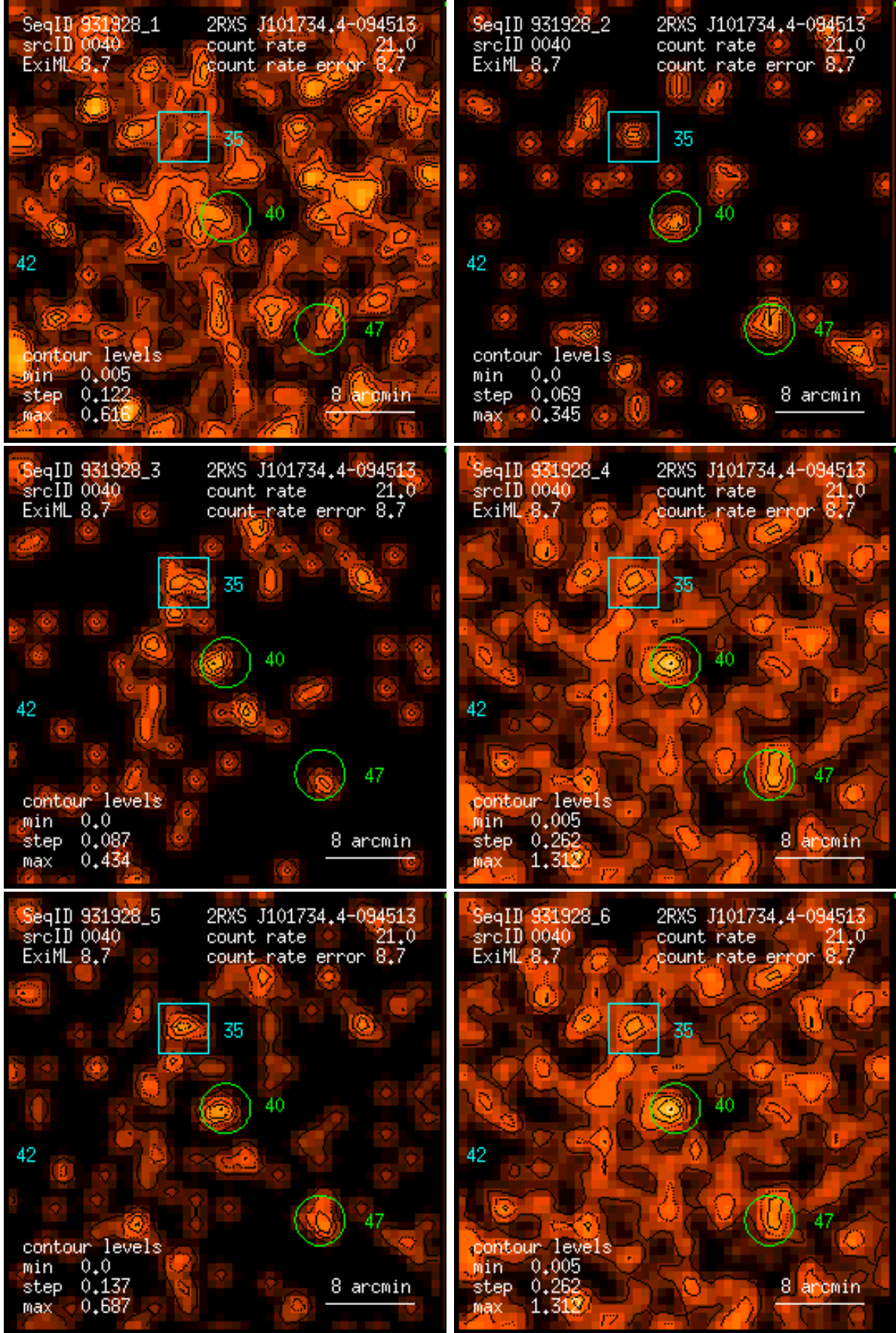
Figure 40: RASS 931928: detection 0040: band rate images, Gaussian filter: (1) PSPC channels 11 – 41, (2) 52 – 90, (3) 91 – 201, (4) 11 – 235, (5) 52 – 201, (6) 11 – 201. Broad band rates in counts/ks. Band rate contour levels in counts/ks/arcmin 2 .
