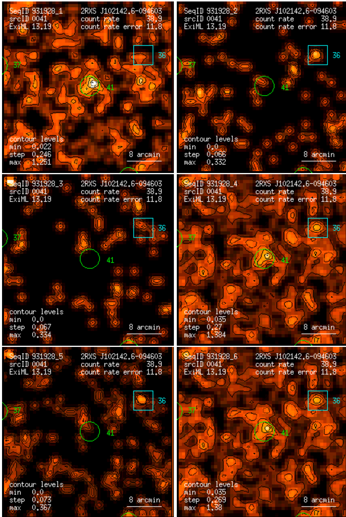
Figure 41: RASS 931928: detection 0041: band rate images, Gaussian filter: (1) PSPC channels 11 – 41, (2) 52 – 90, (3) 91 – 201, (4) 11 – 235, (5) 52 – 201, (6) 11 – 201. Broad band rates in counts/ks. Band rate contour levels in counts/ks/arcmin 2 .
