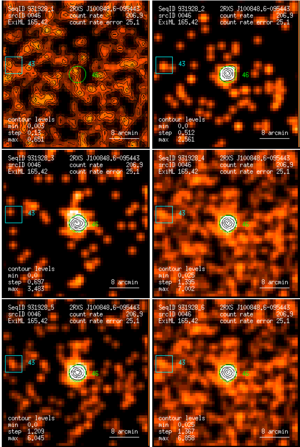
Figure 46: RASS 931928: detection 0046: band rate images, Gaussian filter: (1) PSPC channels 11 – 41, (2) 52 – 90, (3) 91 – 201, (4) 11 – 235, (5) 52 – 201, (6) 11 – 201. Broad band rates in counts/ks. Band rate contour levels in counts/ks/arcmin 2 .
