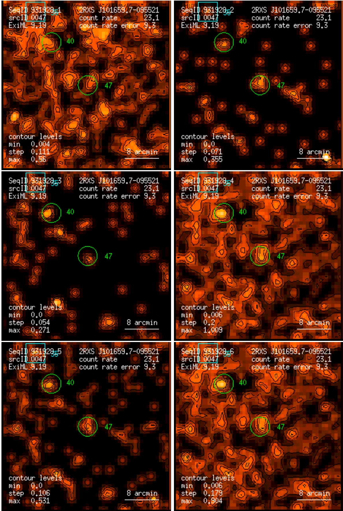
Figure 47: RASS 931928: detection 0047: band rate images, Gaussian filter: (1) PSPC channels 11 – 41, (2) 52 – 90, (3) 91 – 201, (4) 11 – 235, (5) 52 – 201, (6) 11 – 201. Broad band rates in counts/ks. Band rate contour levels in counts/ks/arcmin 2 .
