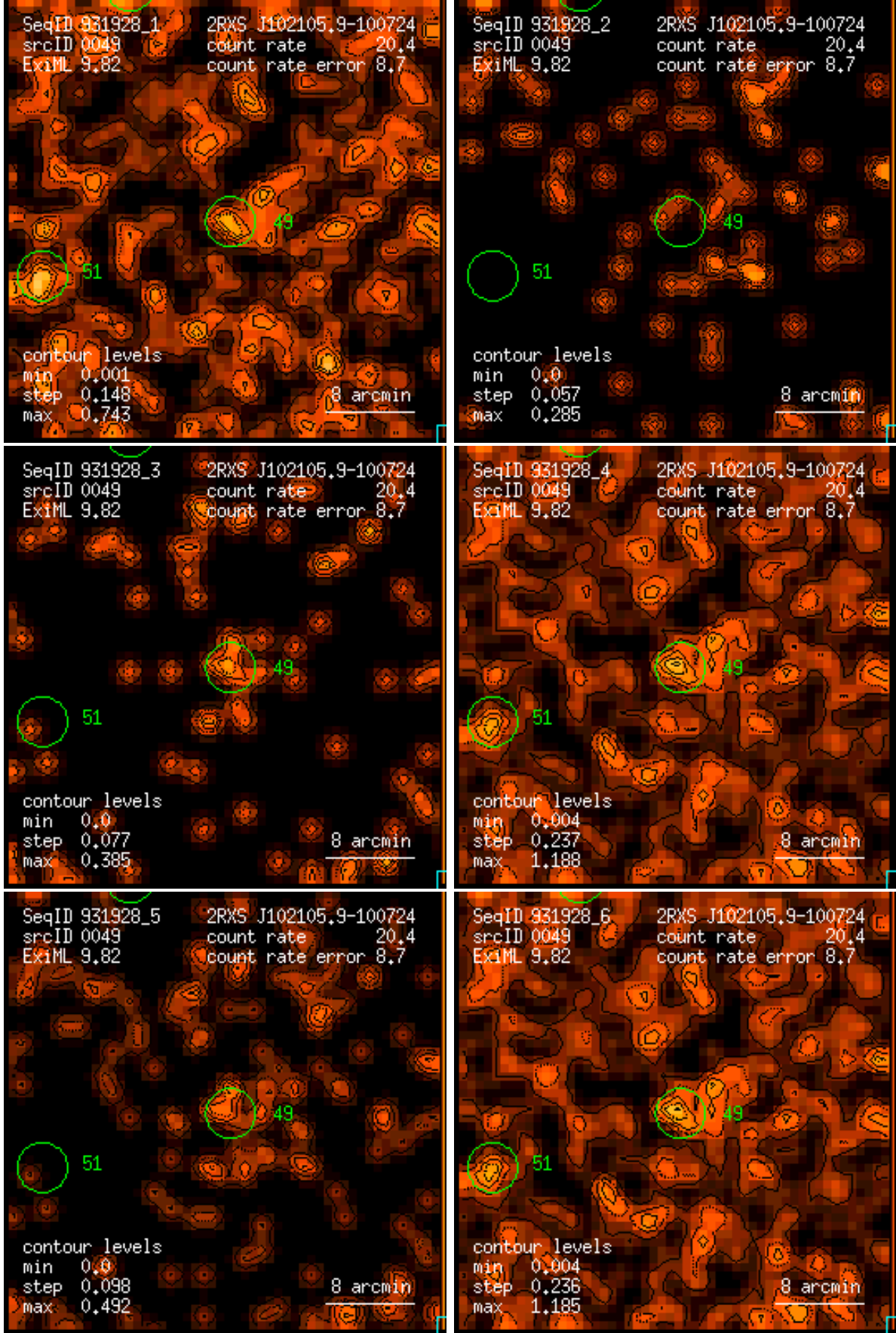
Figure 49: RASS 931928: detection 0049: band rate images, Gaussian filter: (1) PSPC channels 11 – 41, (2) 52 – 90, (3) 91 – 201, (4) 11 – 235, (5) 52 – 201, (6) 11 – 201. Broad band rates in counts/ks. Band rate contour levels in counts/ks/arcmin 2 .
