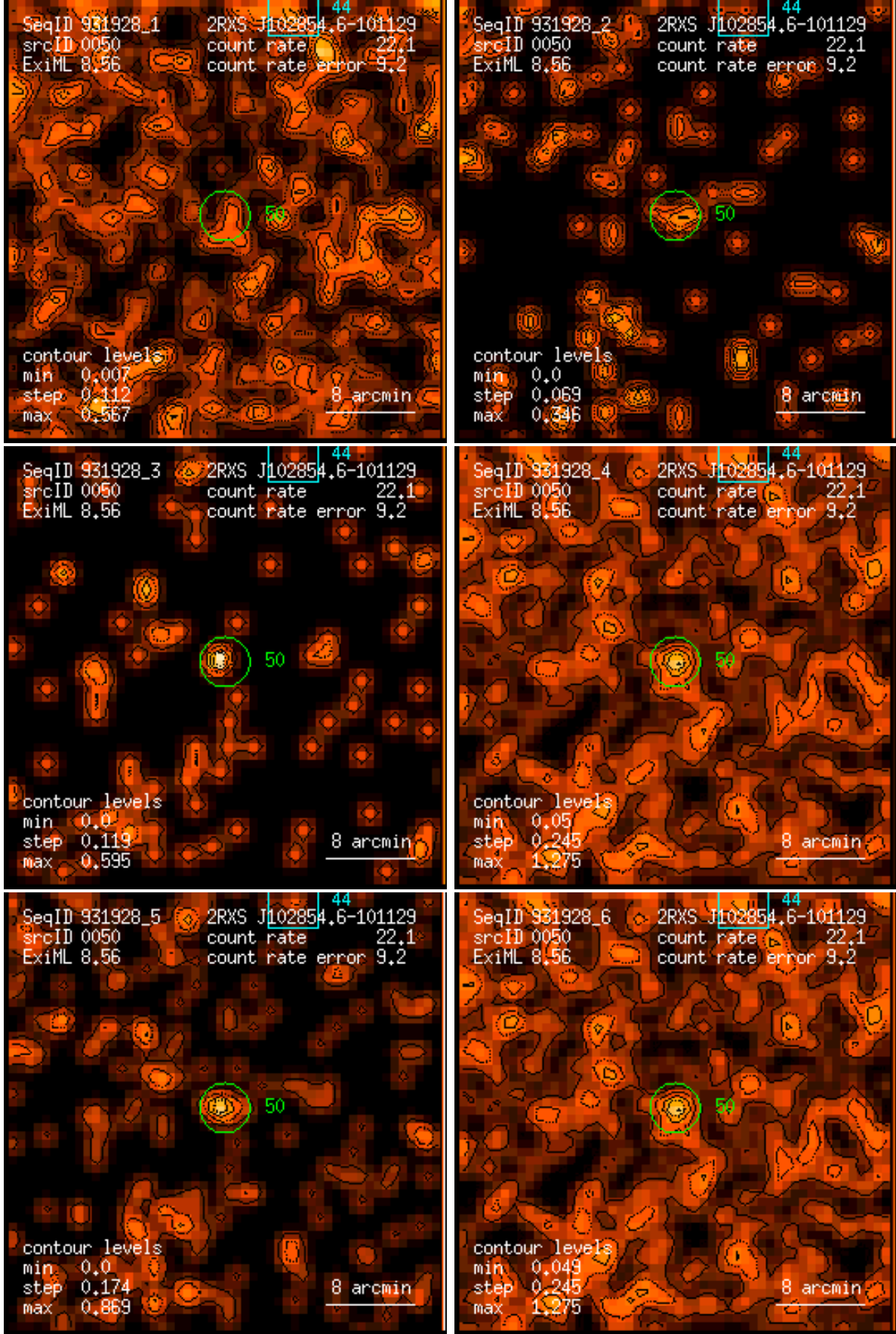
Figure 50: RASS 931928: detection 0050: band rate images, Gaussian filter: (1) PSPC channels 11 – 41, (2) 52 – 90, (3) 91 – 201, (4) 11 – 235, (5) 52 – 201, (6) 11 – 201. Broad band rates in counts/ks. Band rate contour levels in counts/ks/arcmin 2 .
