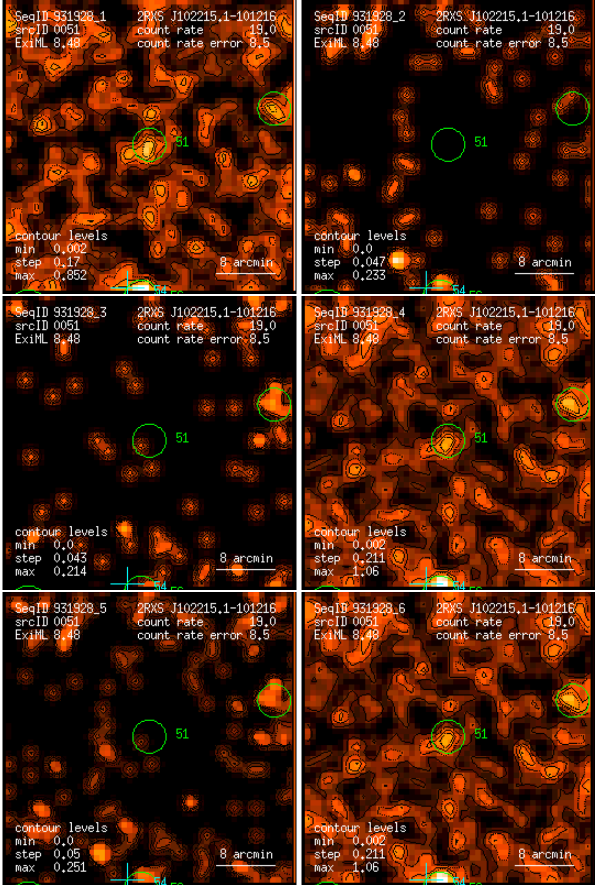
Figure 51: RASS 931928: detection 0051: band rate images, Gaussian filter: (1) PSPC channels 11 – 41, (2) 52 – 90, (3) 91 – 201, (4) 11 – 235, (5) 52 – 201, (6) 11 – 201. Broad band rates in counts/ks. Band rate contour levels in counts/ks/arcmin 2 .
